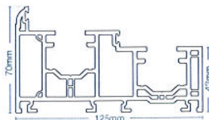
Frame VSW001
