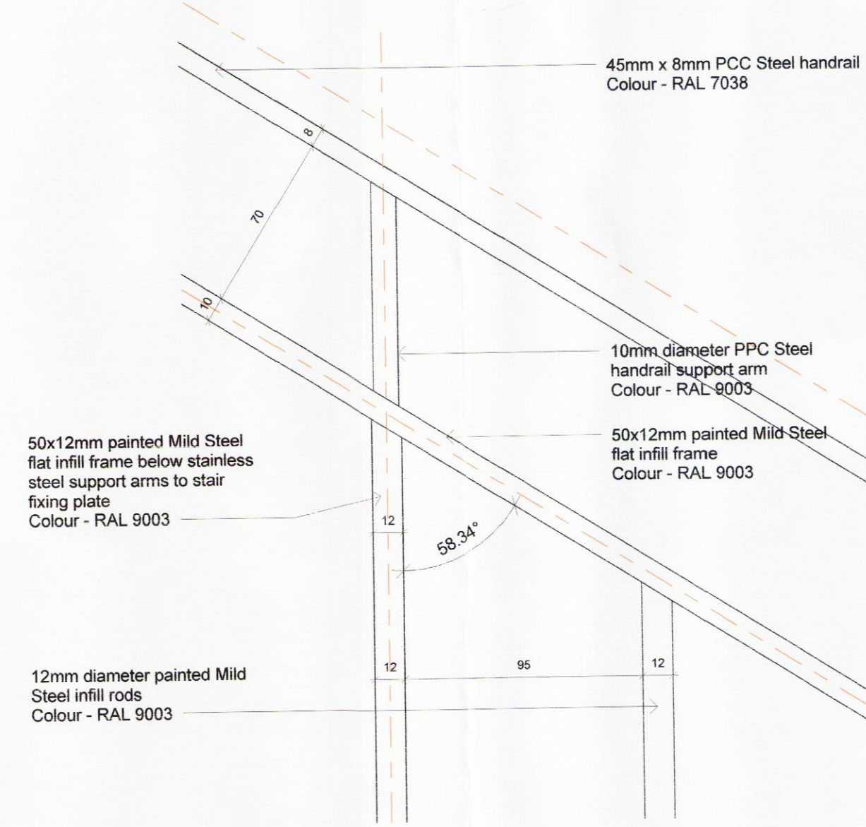
Stair Handrail Support Detail
