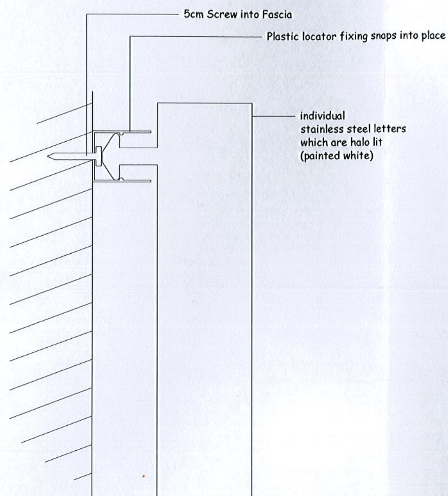
Section Through Proposed Fixing of Sign (Scale 5:1)
