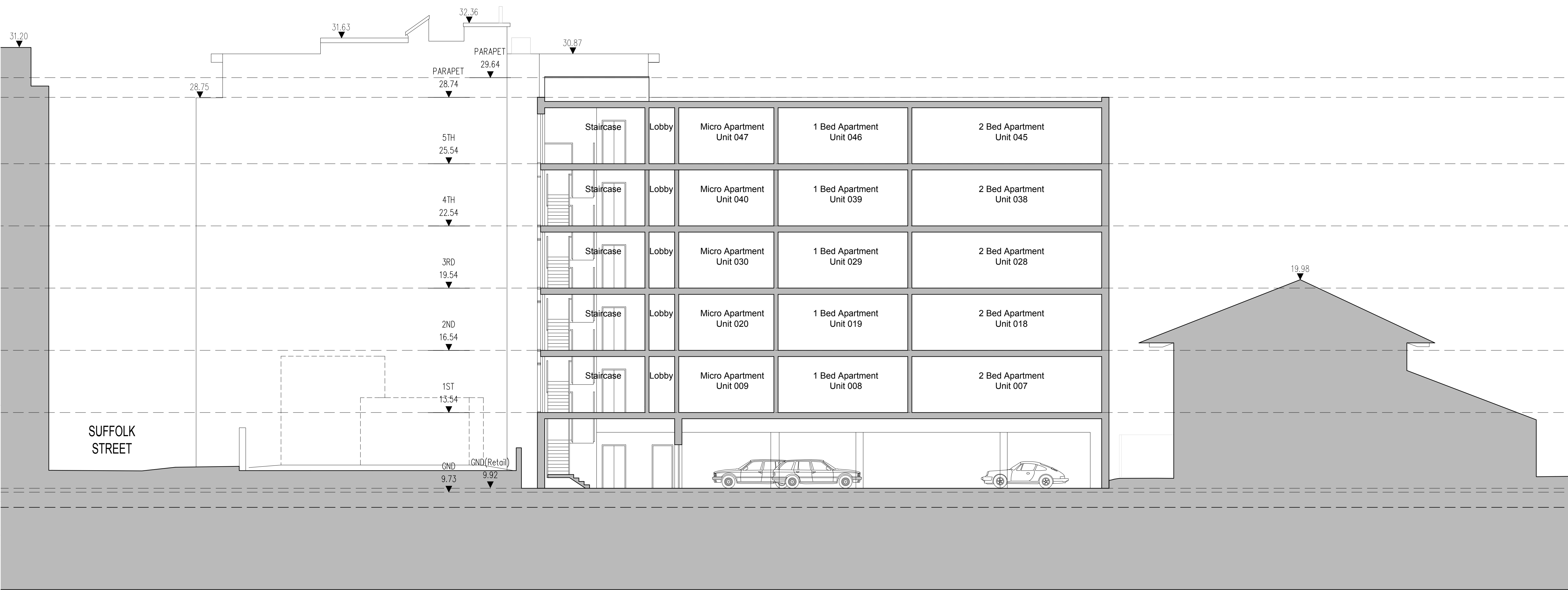
Section B-B
