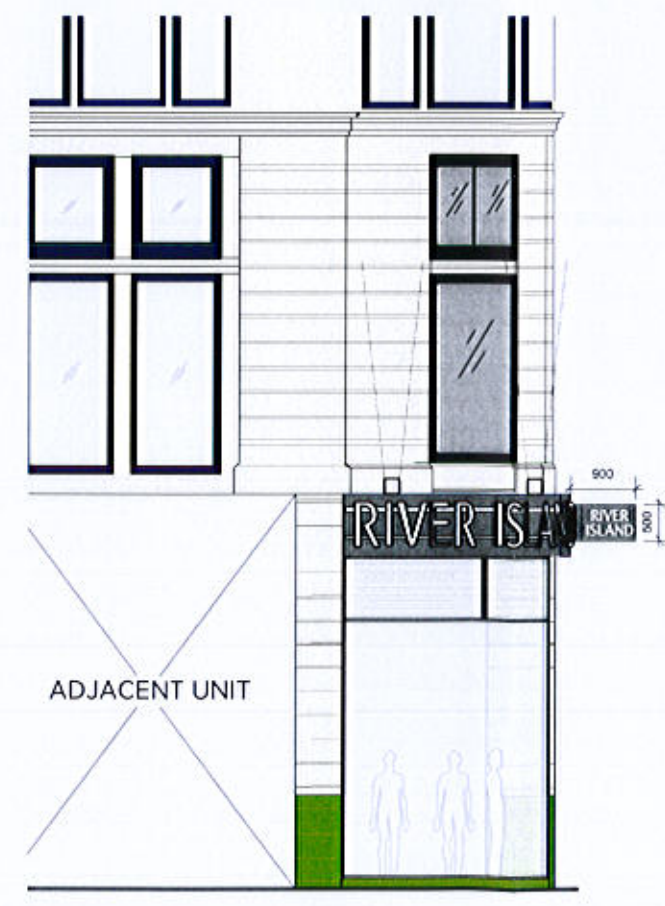
EXISTING SHOPFRONT RETURN ELEVATION @ 1:50
