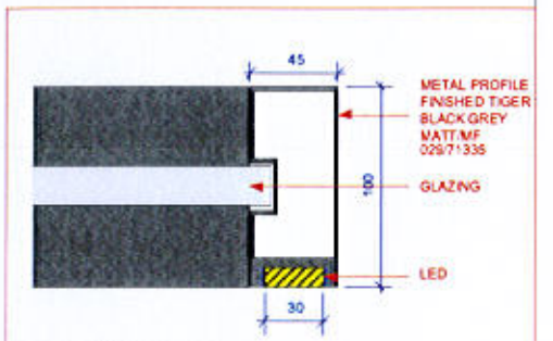
DETAIL 2 @ 1:2
