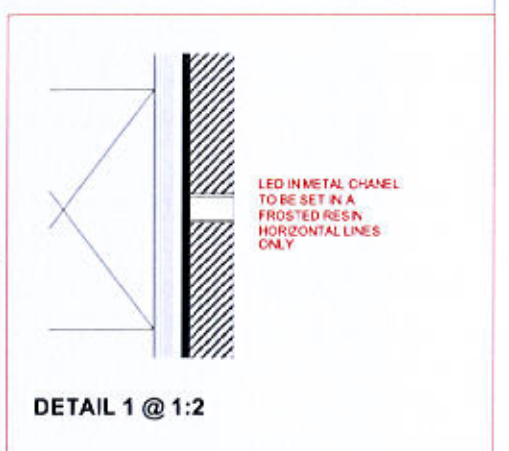
DETAIL 1 @ 1:2
