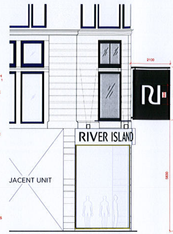
PROPOSED SHOPFRONT RETURN ELEVATION @ 1:50
