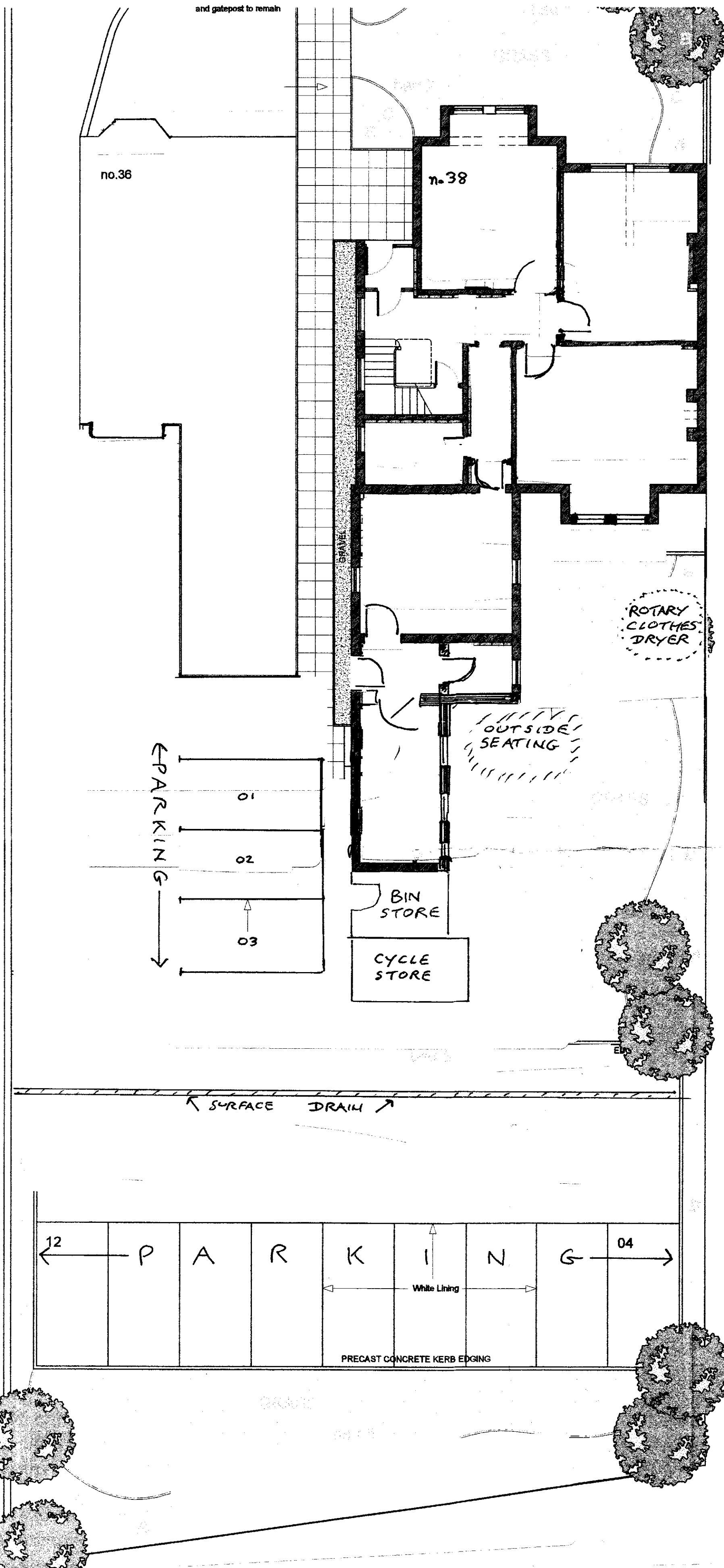
Proposed Site Plan
