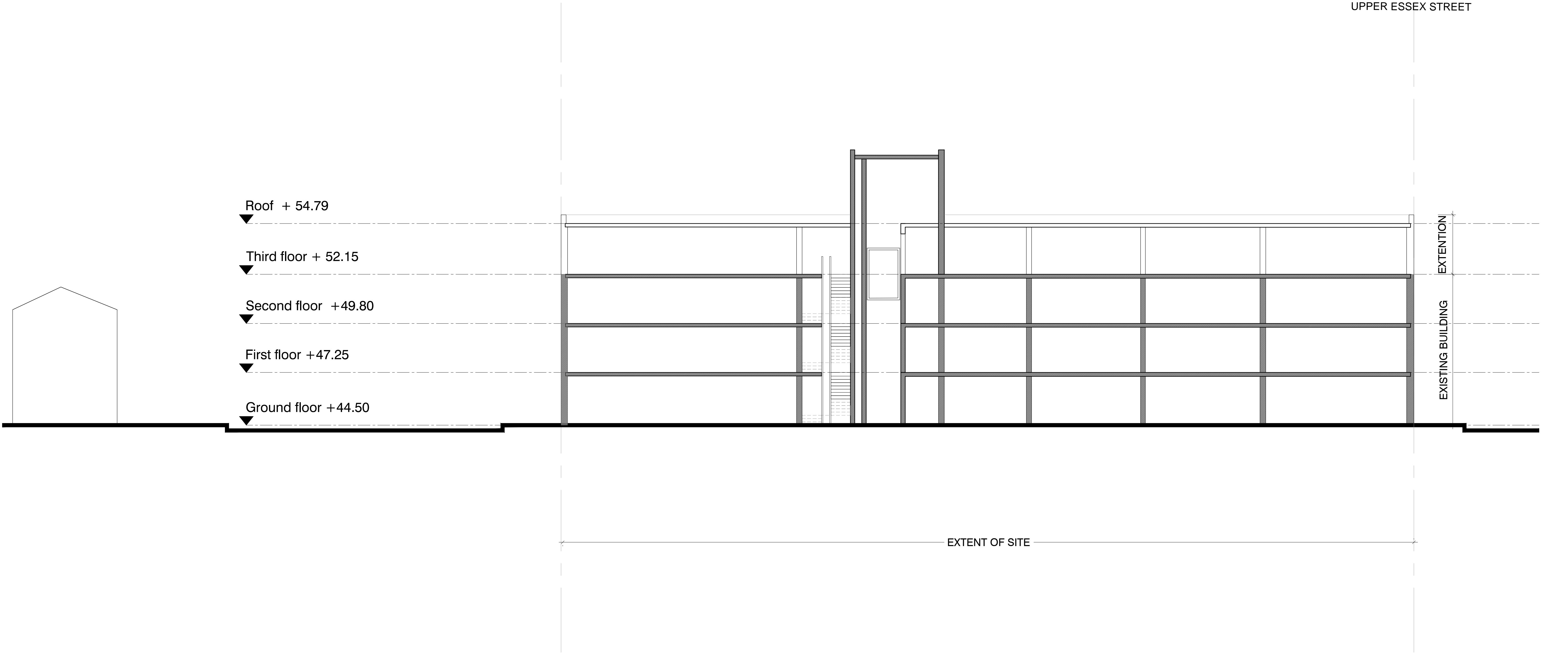
PROPOSED SECTION
