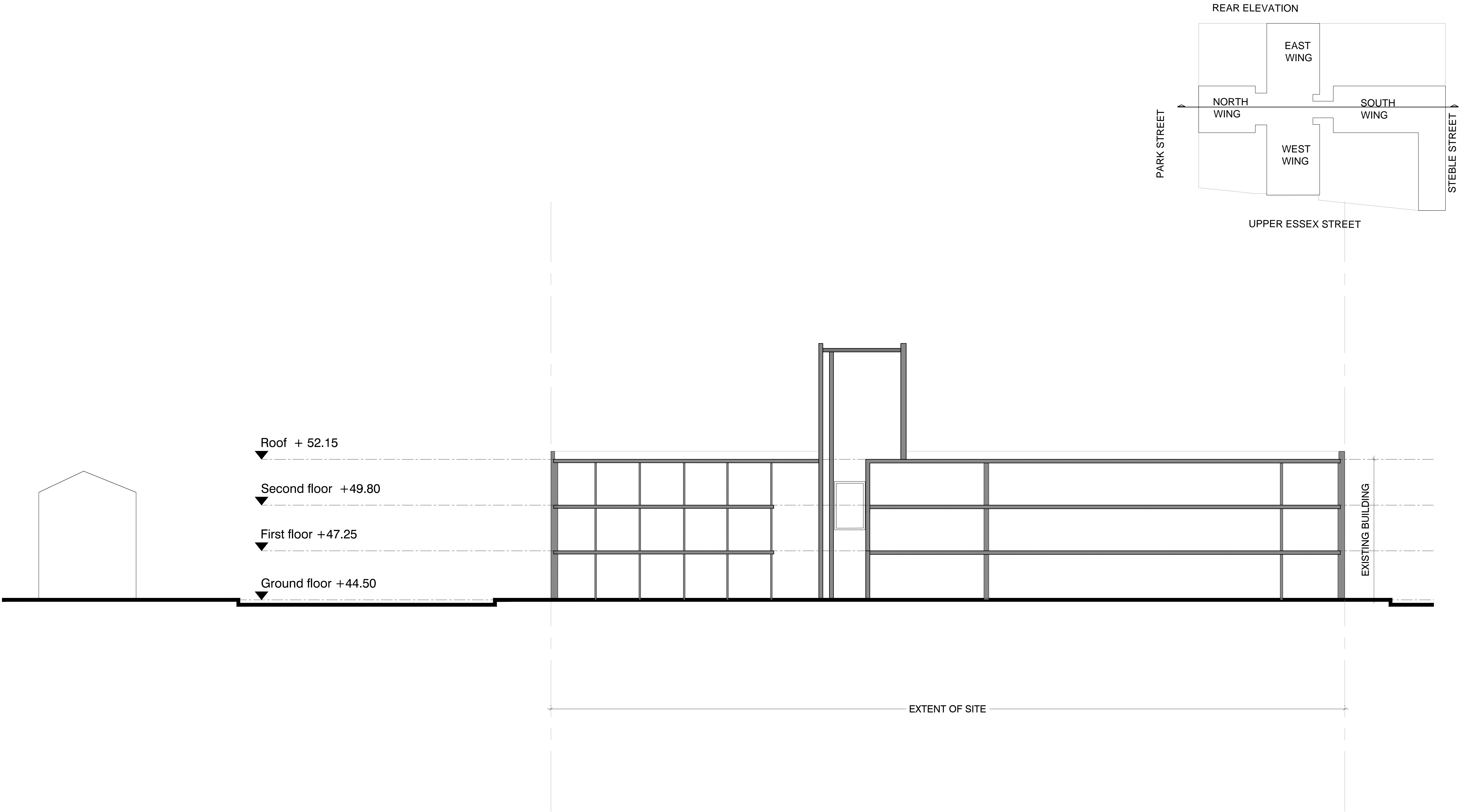
EXISTING SECTION
