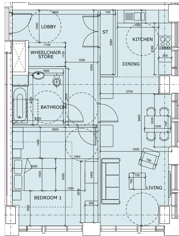
Type G - 1 Bedroom Accessible
