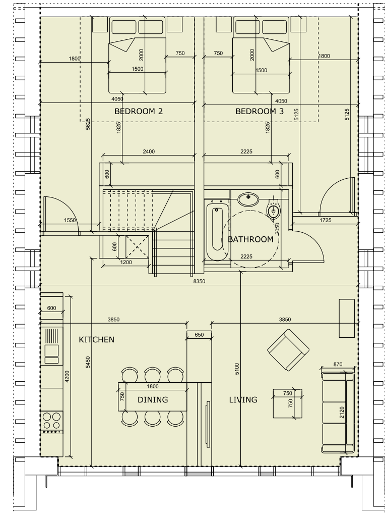
Type F - 3 Bedroom Duplex (Upper)
