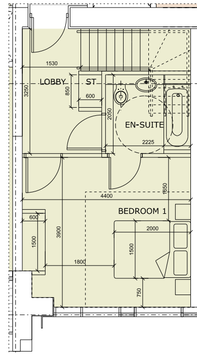
Type F - 3 Bedroom Duplex (Lower)
