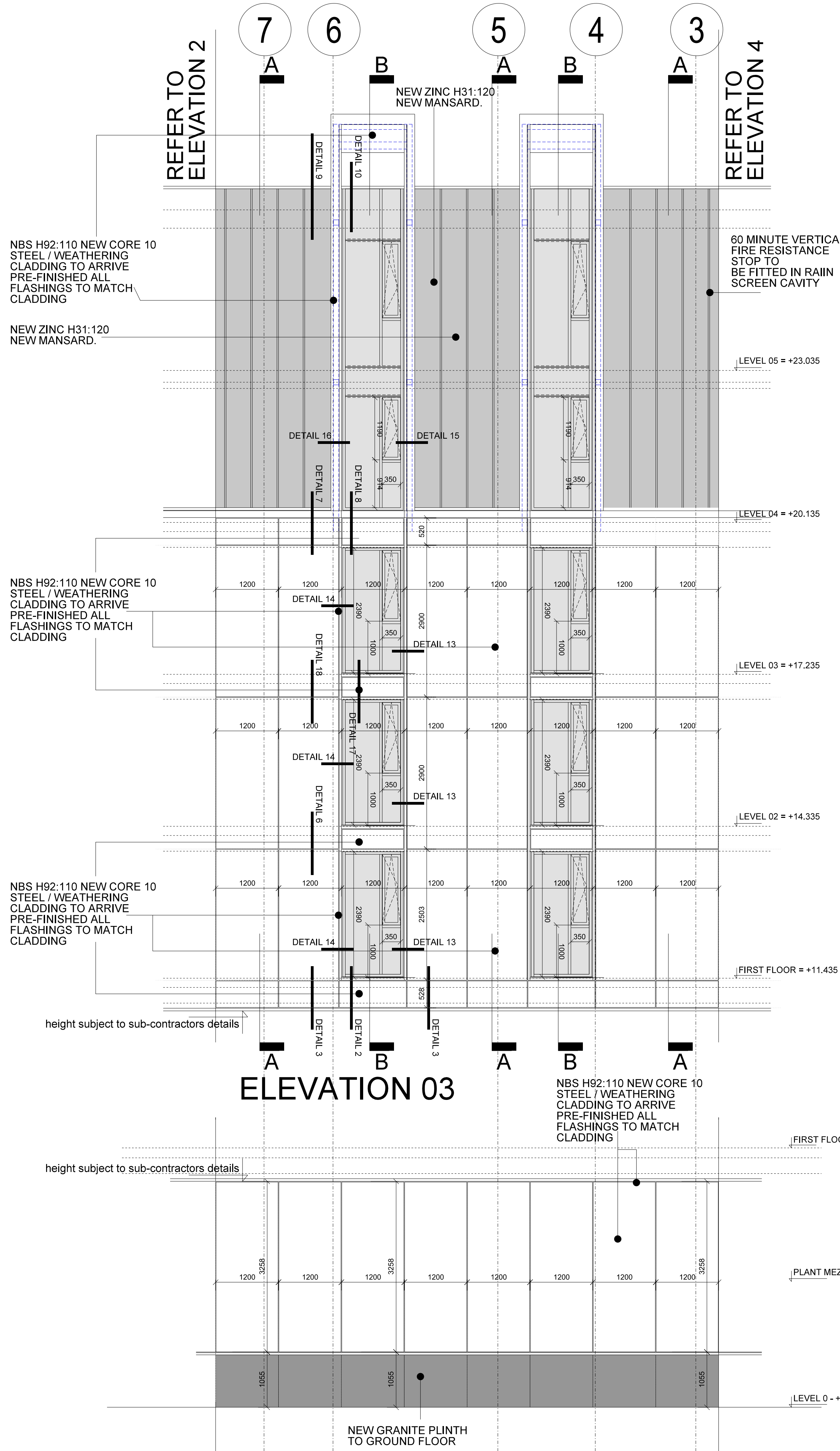
ELEVATION 03A - ground floor
