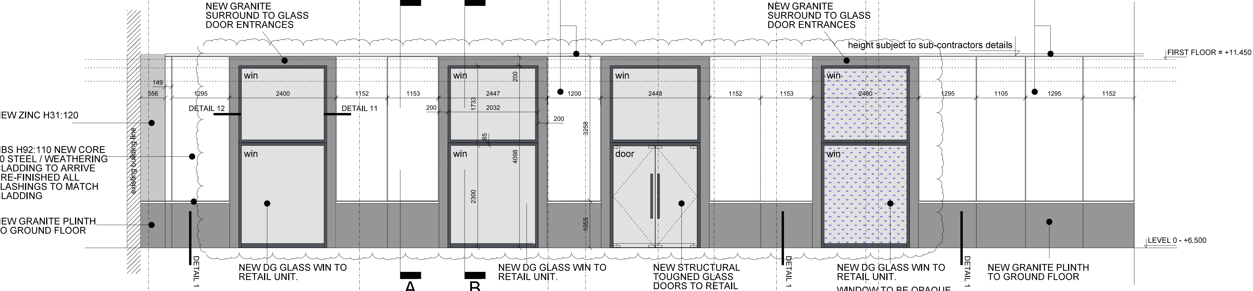
ELEVATION 01A - ground floor
