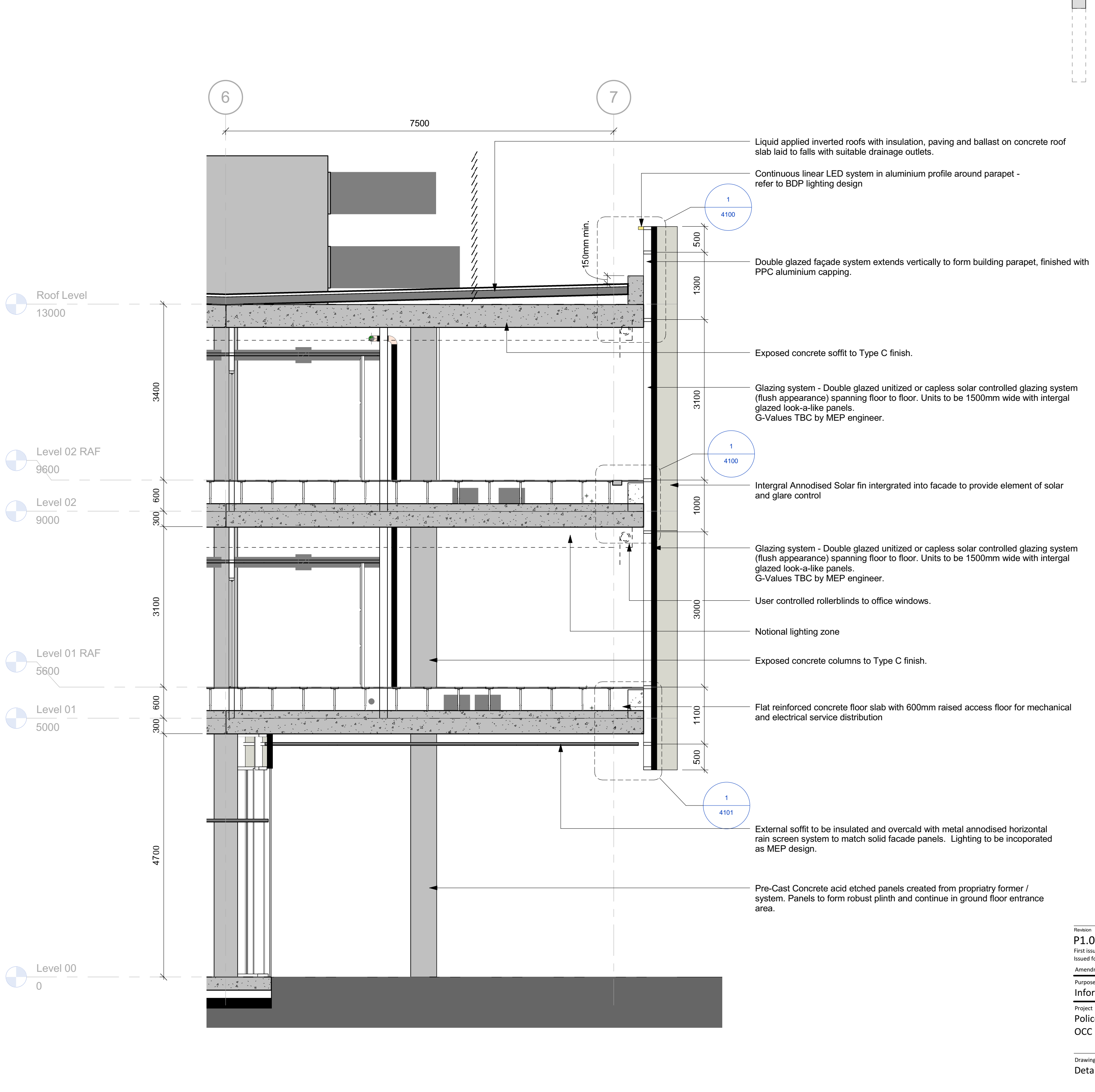
02 - Horizontal rainscreen soffit.
