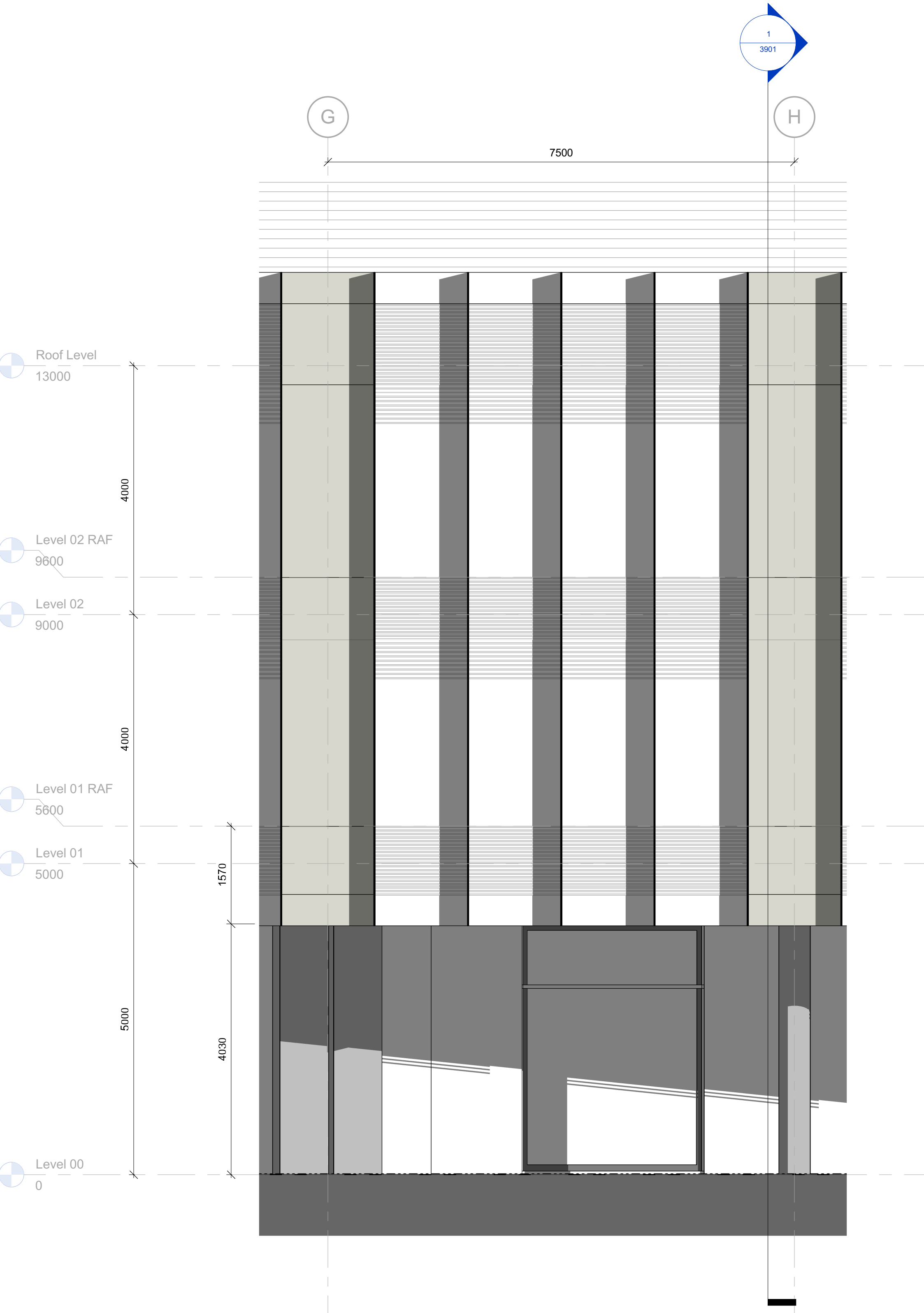
01 - Capless / Unitized Glazing System with fritted glass. System to intergal fins / solid, openable panels
