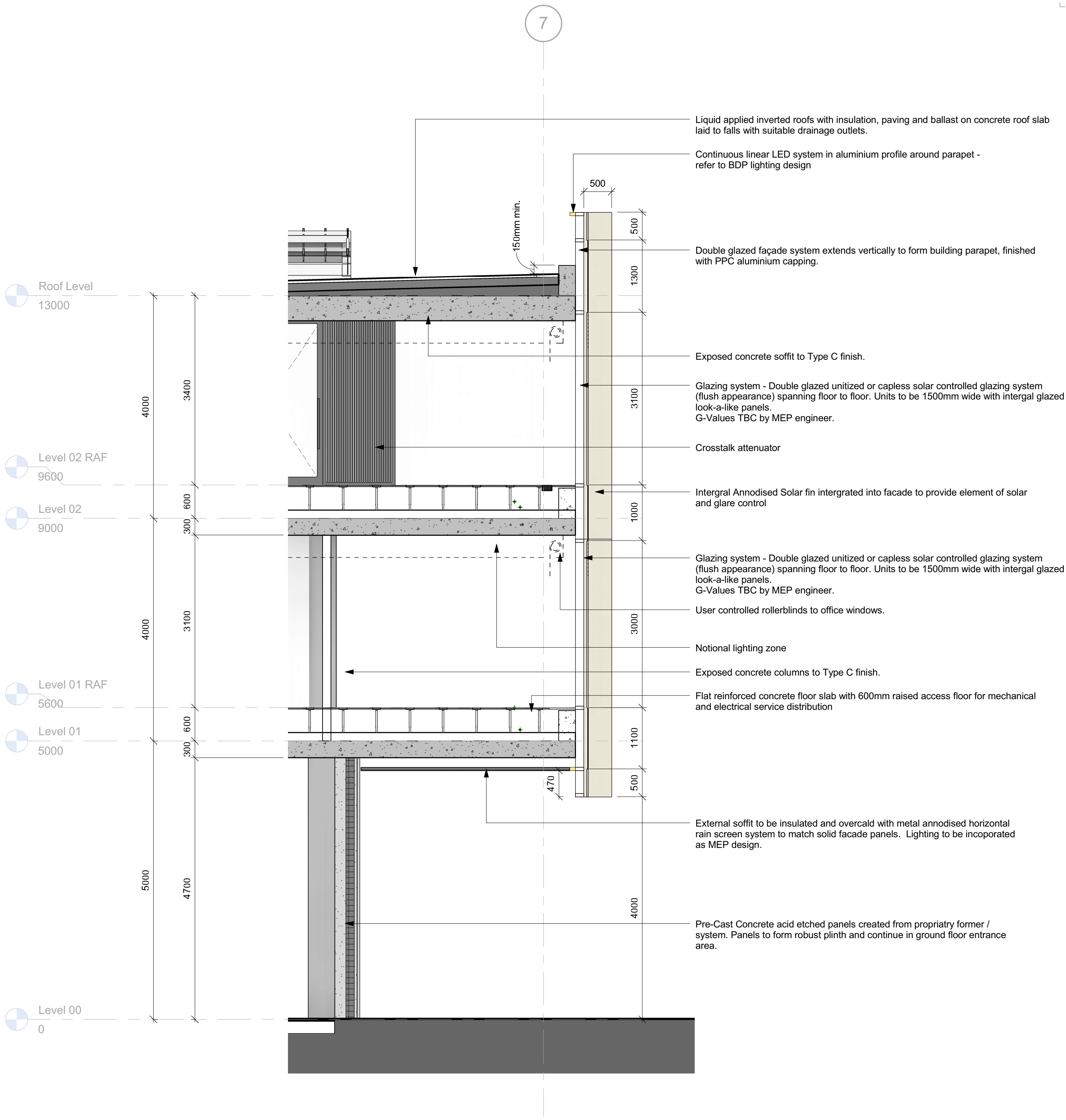
Typical Bay - West Facade Section
