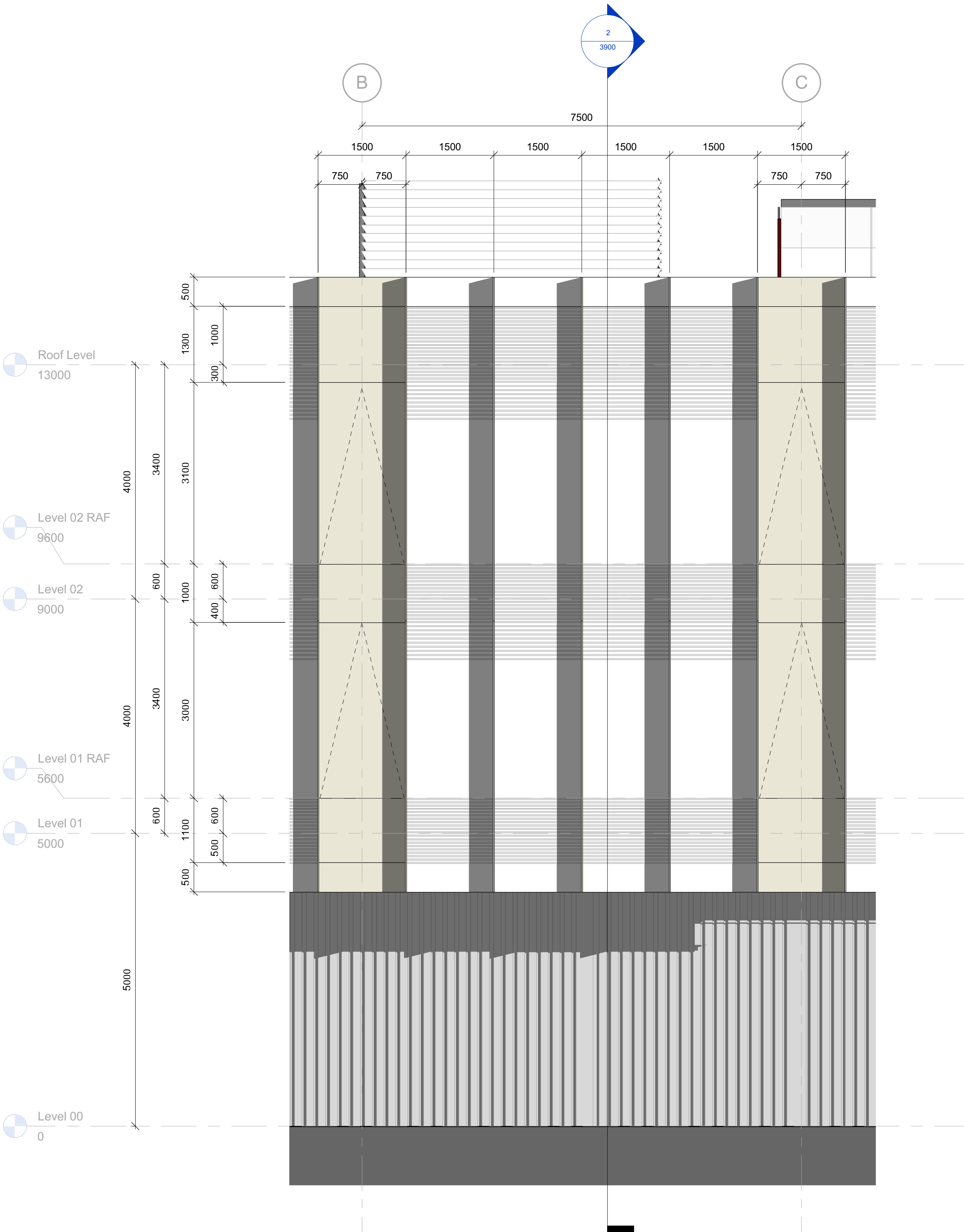
Typical Bay - West Facade Elevation
