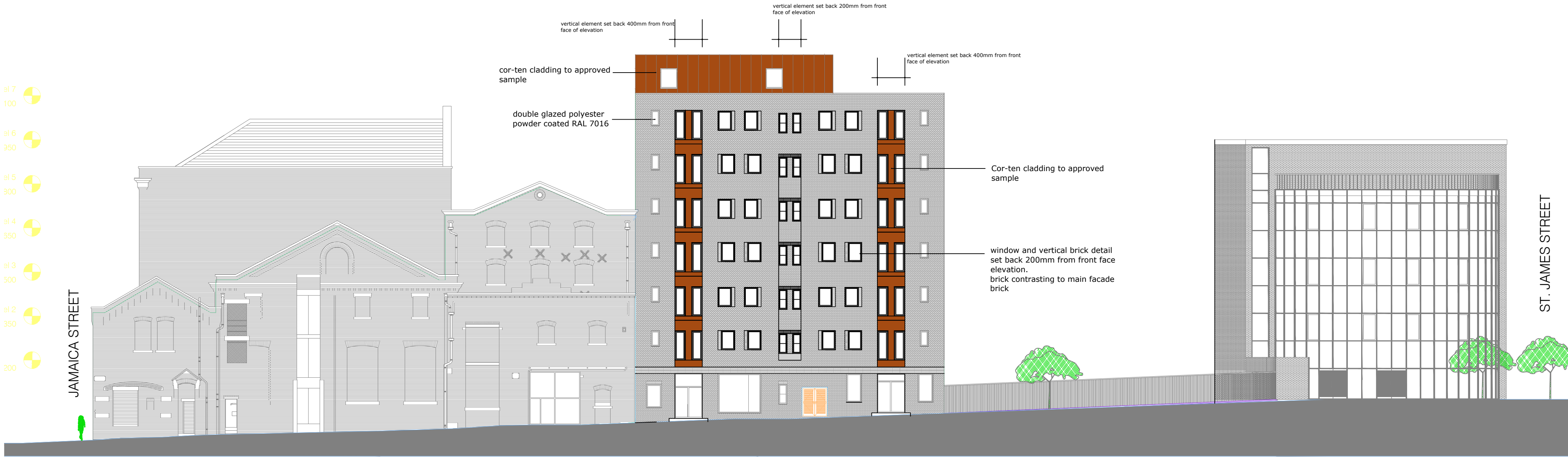
NORFOLK STREET ELEVATION
