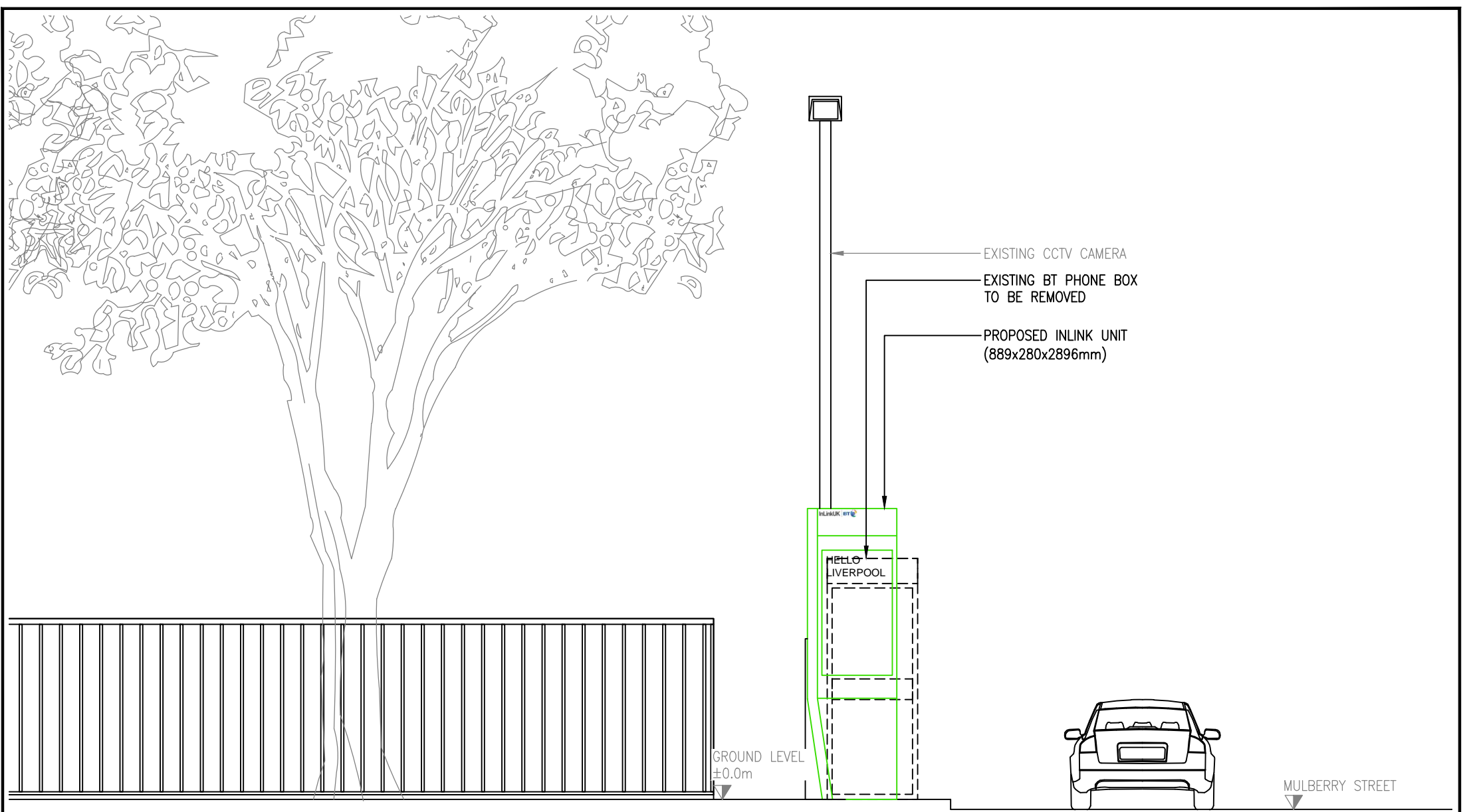
SITE ELEVATION SCALE 1:50
