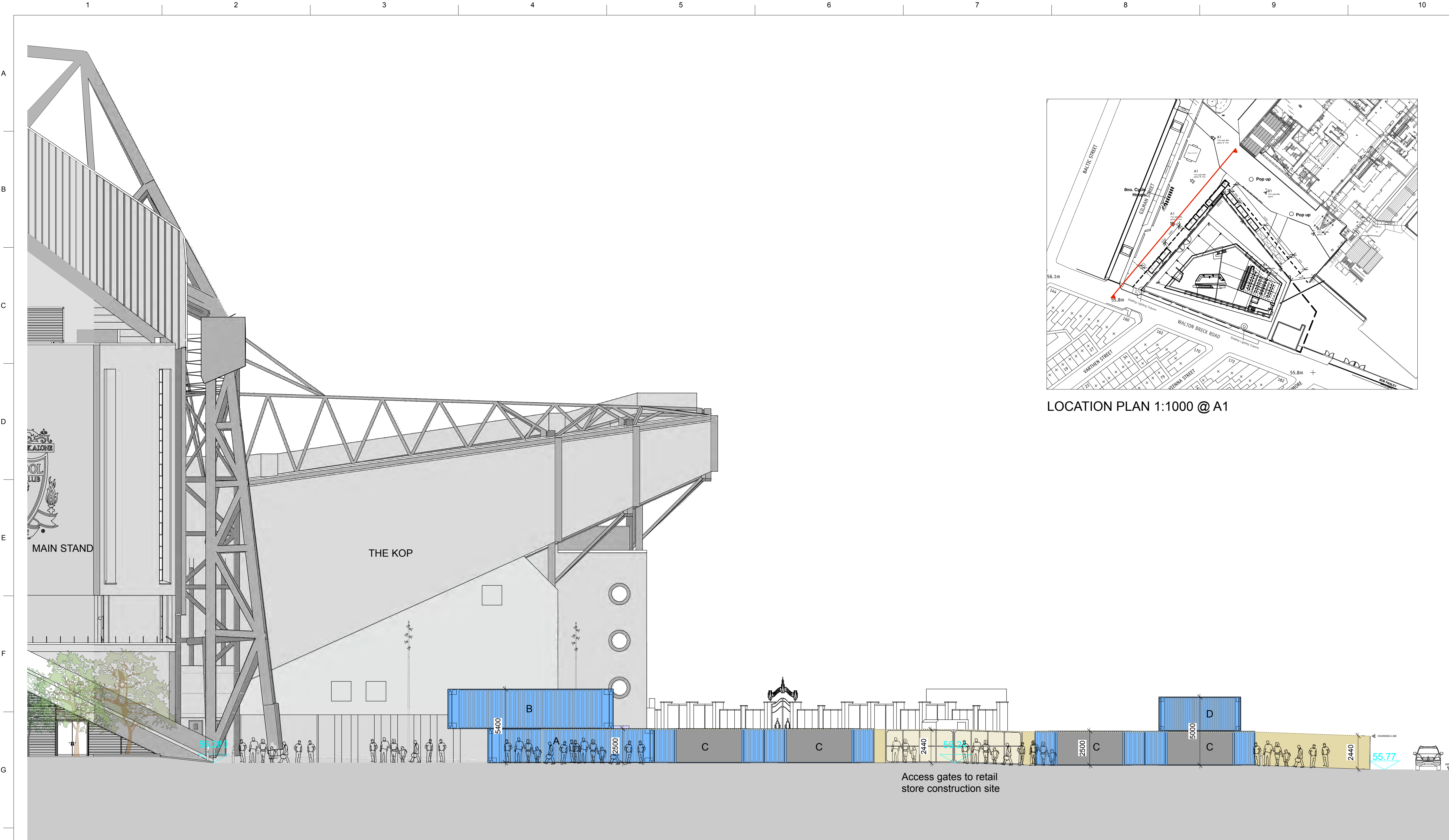
SECTION FROM WALTON BRECK ROAD TO THE MAIN STAND SHOWING EXTENT OF CONTAINERS
