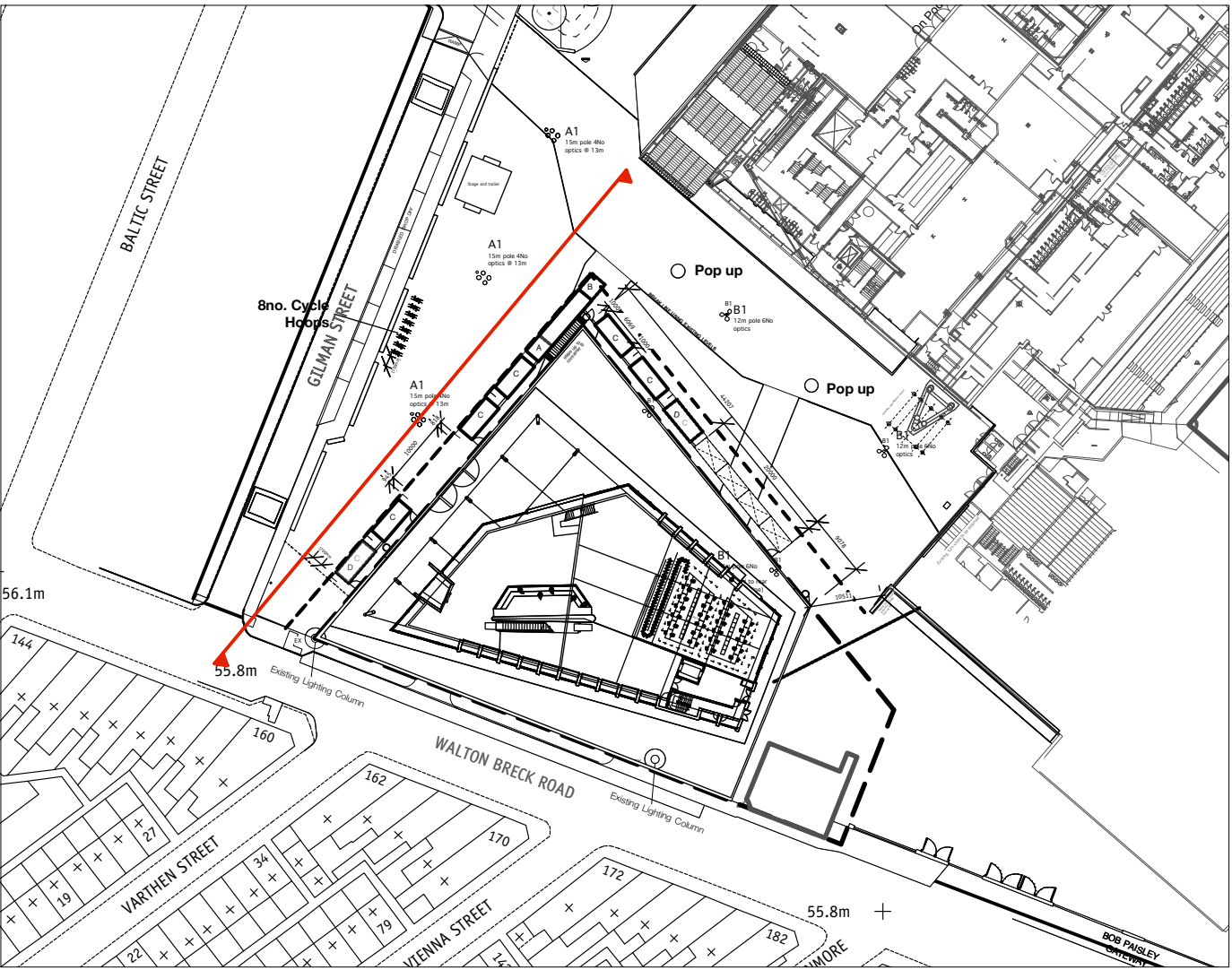
LOCATION PLAN 1:1000 @ A1
