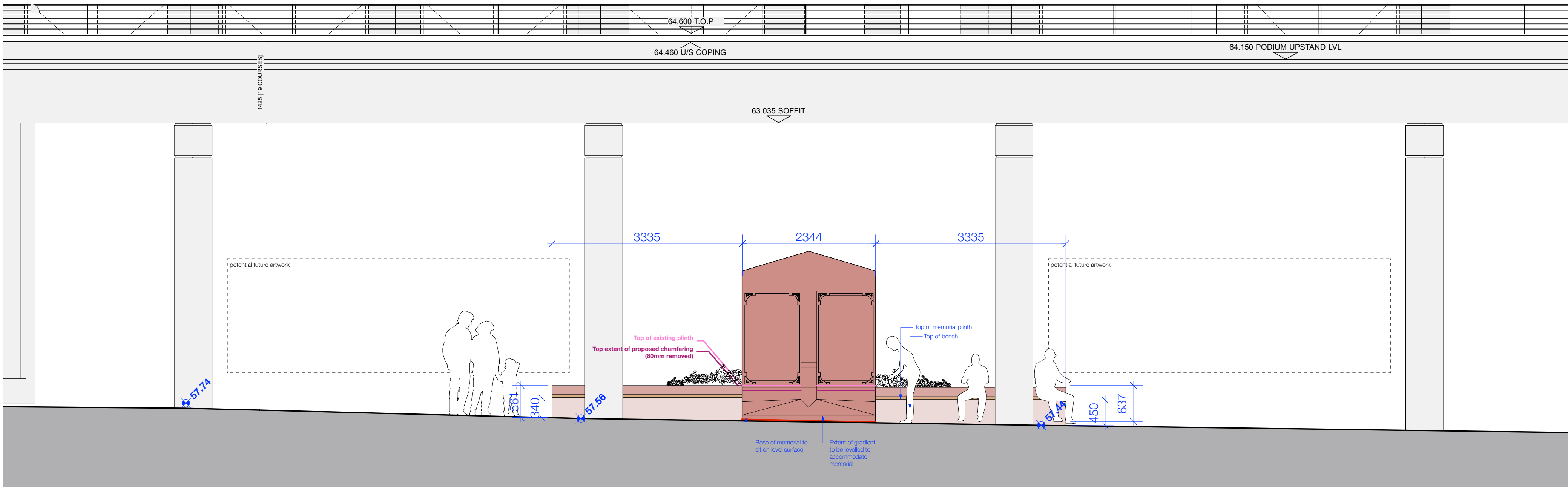
A-A Memorial Elevation - 1:50
