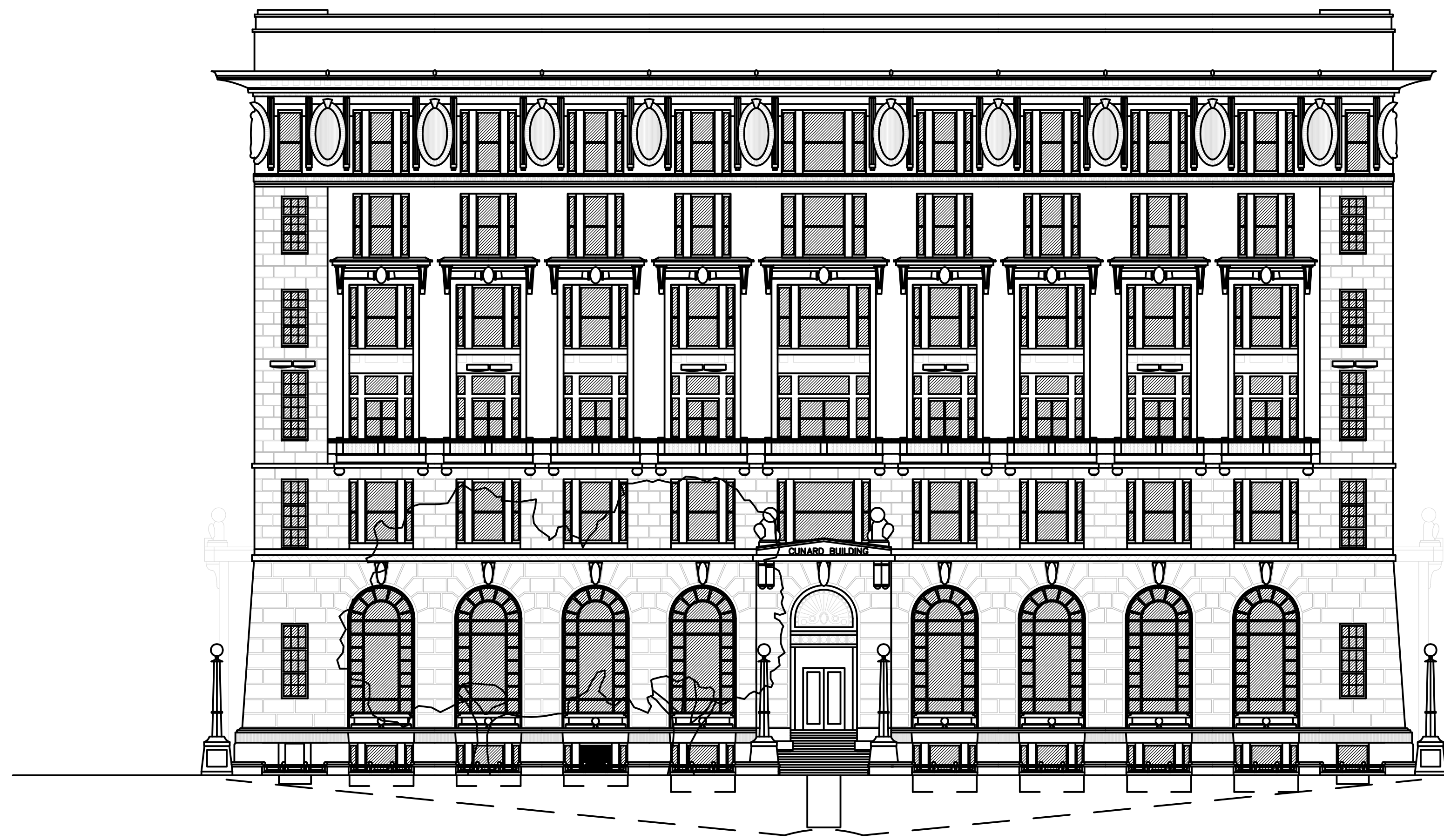
The Strand Elevation
