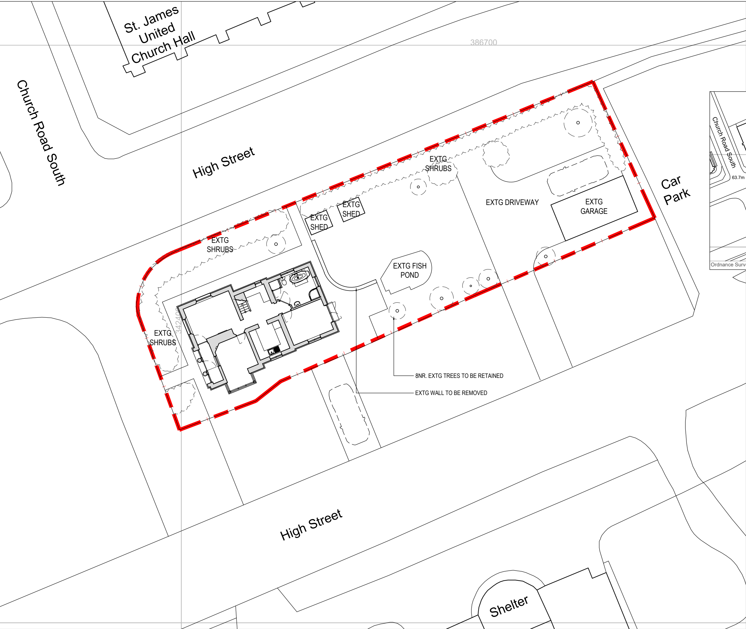
EXISTING SITE PLAN scale 1:200
