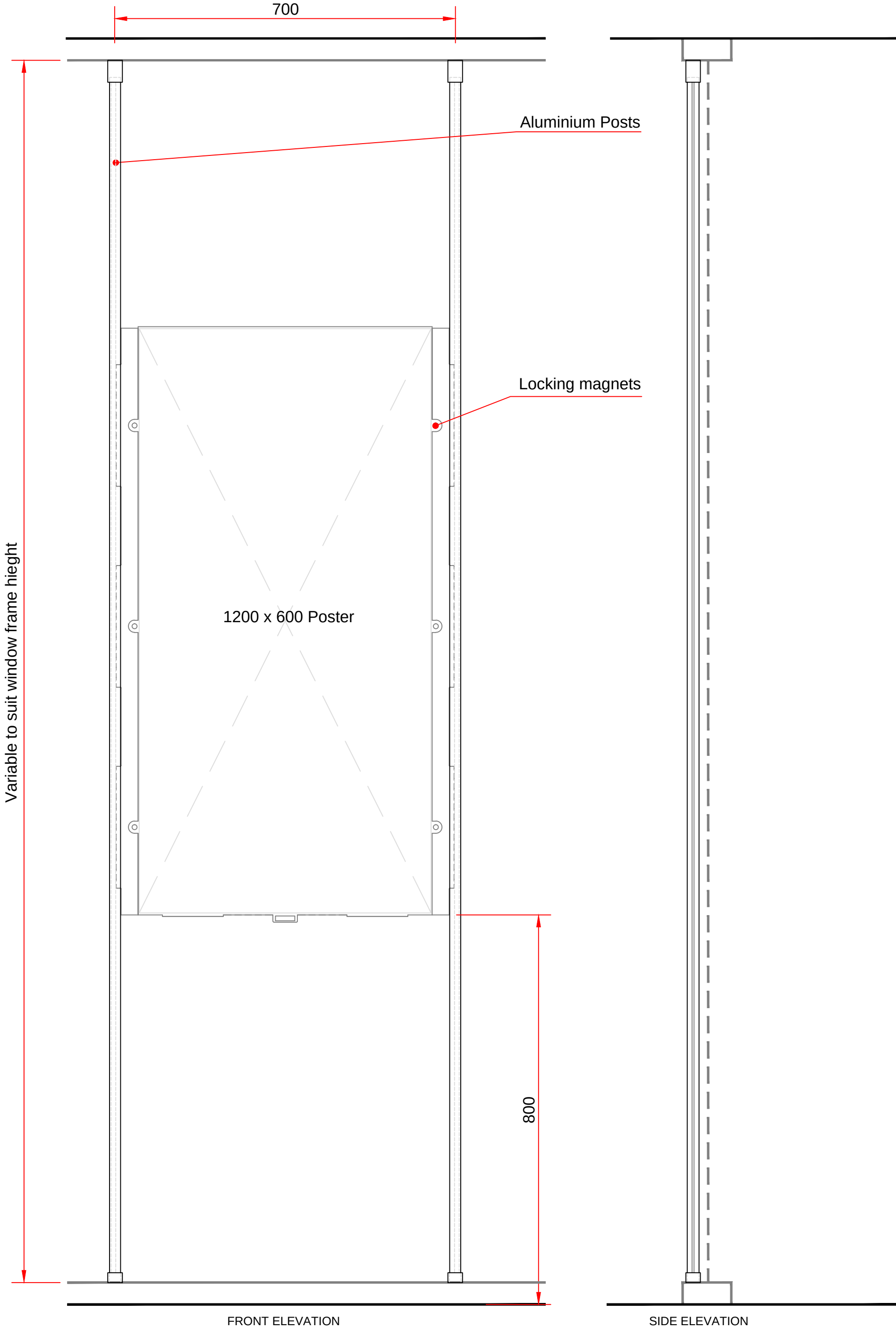
FRONT ELEVATION
