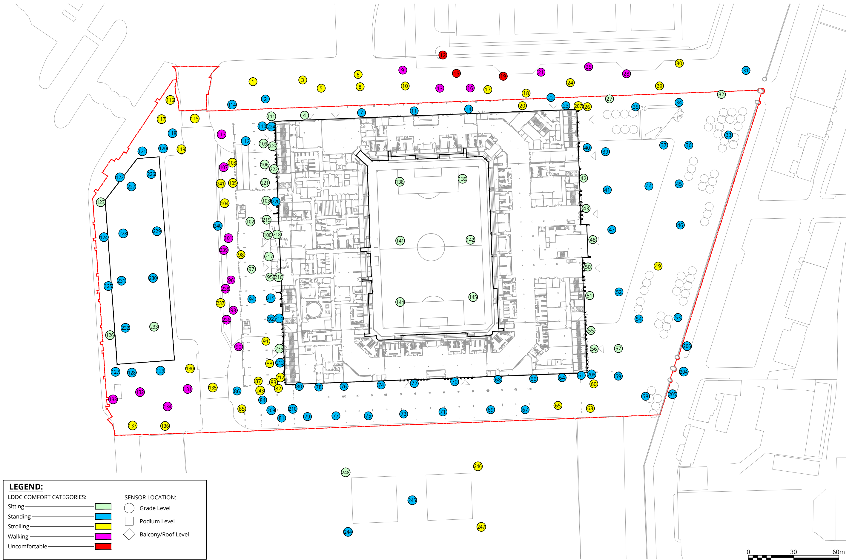
Pedestrian Wind Comfort Conditions - Ground Floor Configuration 4: Proposed Development with Cumulative Surrounding Buildings, Proposed Landscaping and Design Interventions Windiest Season
