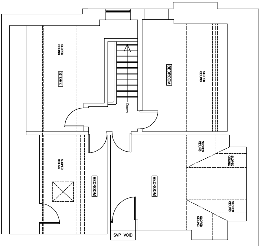
EXISTING SECOND FLOOR PLAN Scale 1:50 0 500mm 1500mm 2000mm 1000mm
