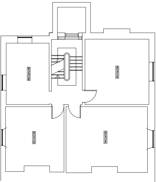
EXISTING FIRST FLOOR PLAN Scale 1:50 0 500mm 1500mm 2000mm 1000mm
