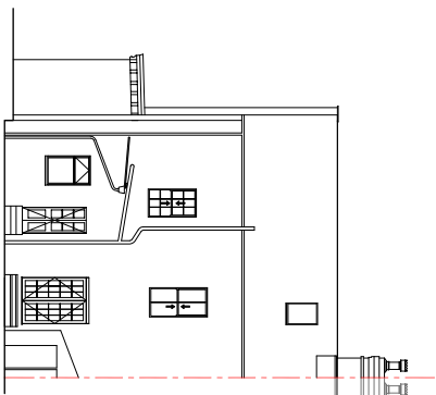
EXISTING REAR ELEVATION Scale 1:100 0 1000mm 3000mm 4000mm 2000mm
