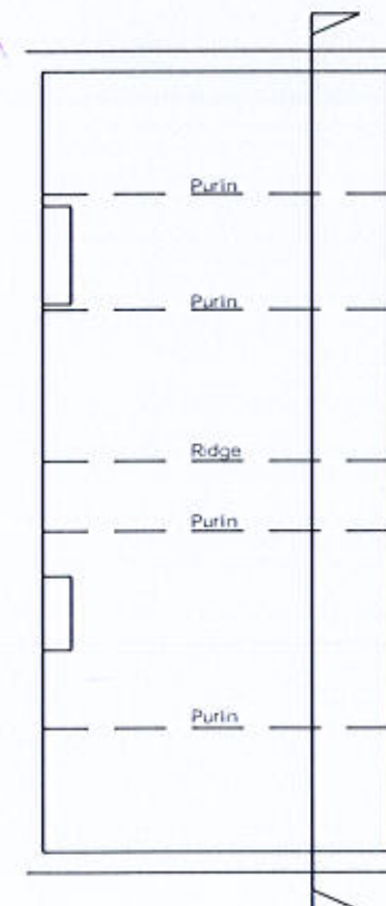
Existing Roof Layout
