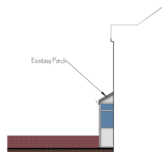
4 Right Side Elevation 1 : 100
