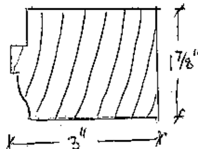
BOTTOM RAIL
