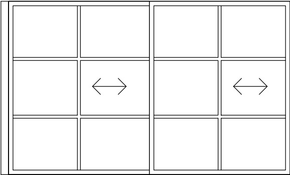
SW01; SW02; SW03 New traditional timber box sash windows, single glazed, with narrow moulded glazing bars.
