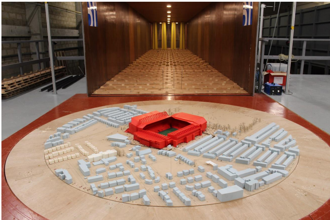
Figure 12.36 Proposed Scheme with Cumulative Surrounding Buildings and Existing Landscaping Scheme (Configuration 3) – View in the Wind Tunnel (from the south)
