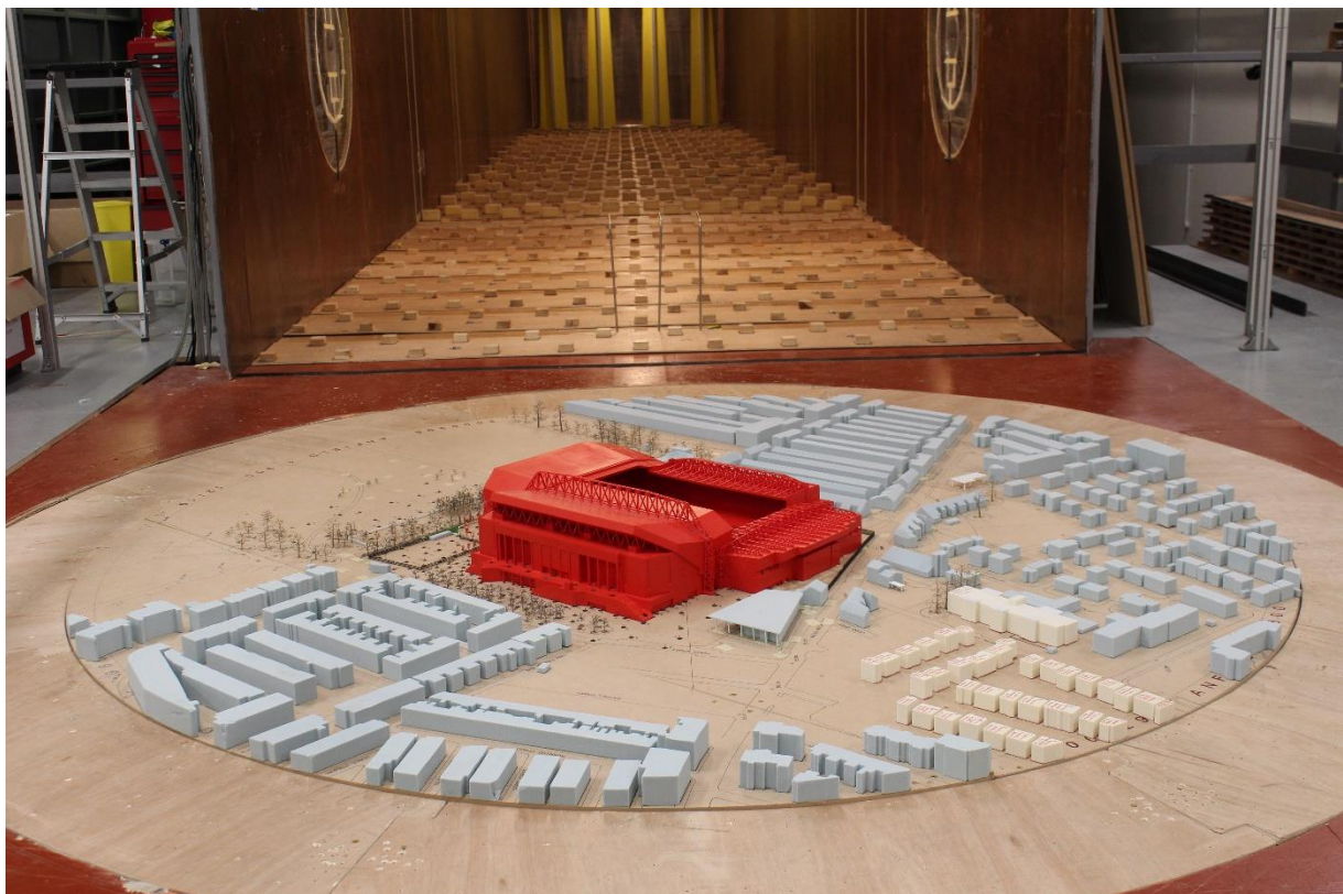
Figure 12.45 Proposed Scheme with Cumulative Surrounding Buildings, Existing and Proposed Landscaping Scheme (Configuration 5) – View in the Wind Tunnel (from the west)
