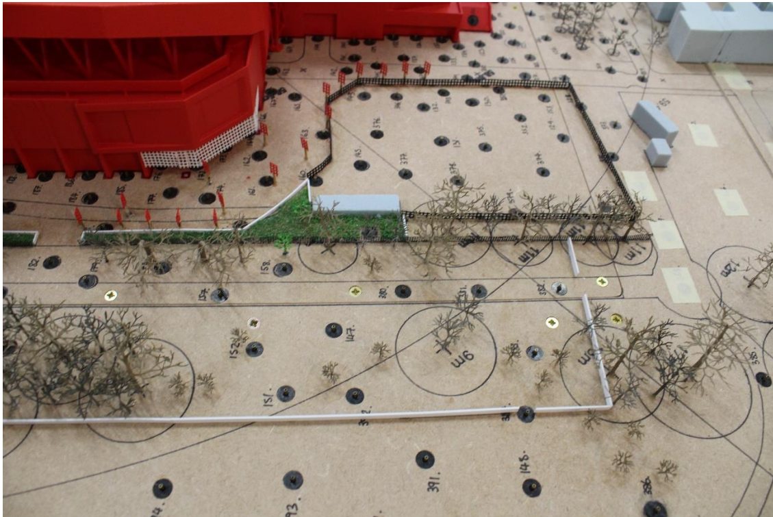
Figure 12.42 Proposed Landscaping Scheme – (Wind Tunnel model photo)
