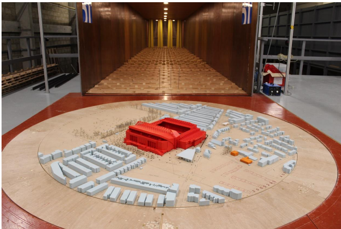
Figure 12.33 Existing Site with Existing Surrounding Buildings and Existing Landscaping Scheme (Configuration 1) – View in the Wind Tunnel (from the west)
