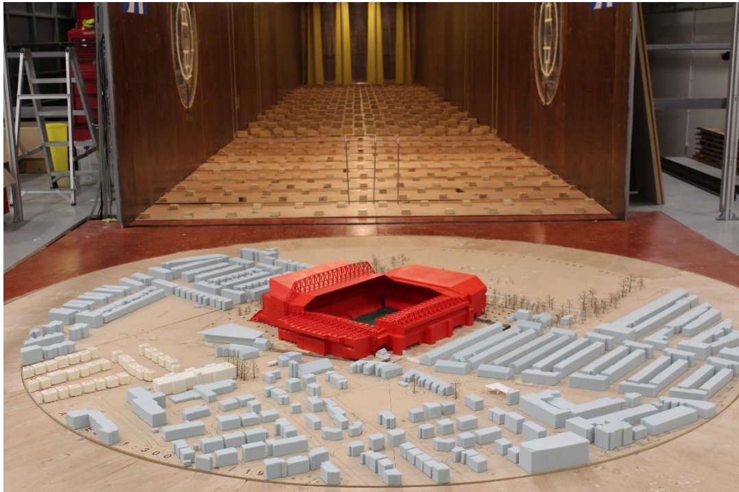
Figure 12.44 Proposed Scheme with Cumulative Surrounding Buildings, Existing and Proposed Landscaping Scheme (Configuration 5) – View in the Wind Tunnel (from the south)
