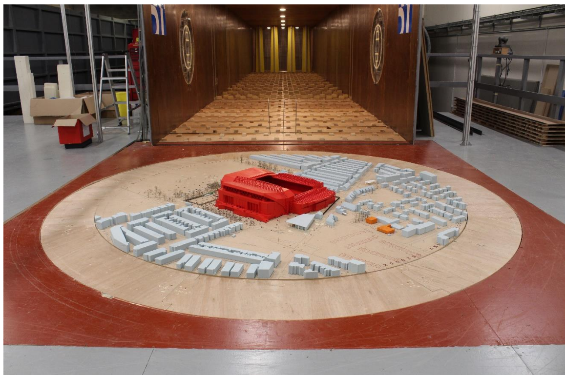
Figure 12.39 Proposed Scheme with Existing Surrounding Buildings, Existing and Proposed Landscaping Scheme (Configuration 4) – View in the Wind Tunnel (from the west)
