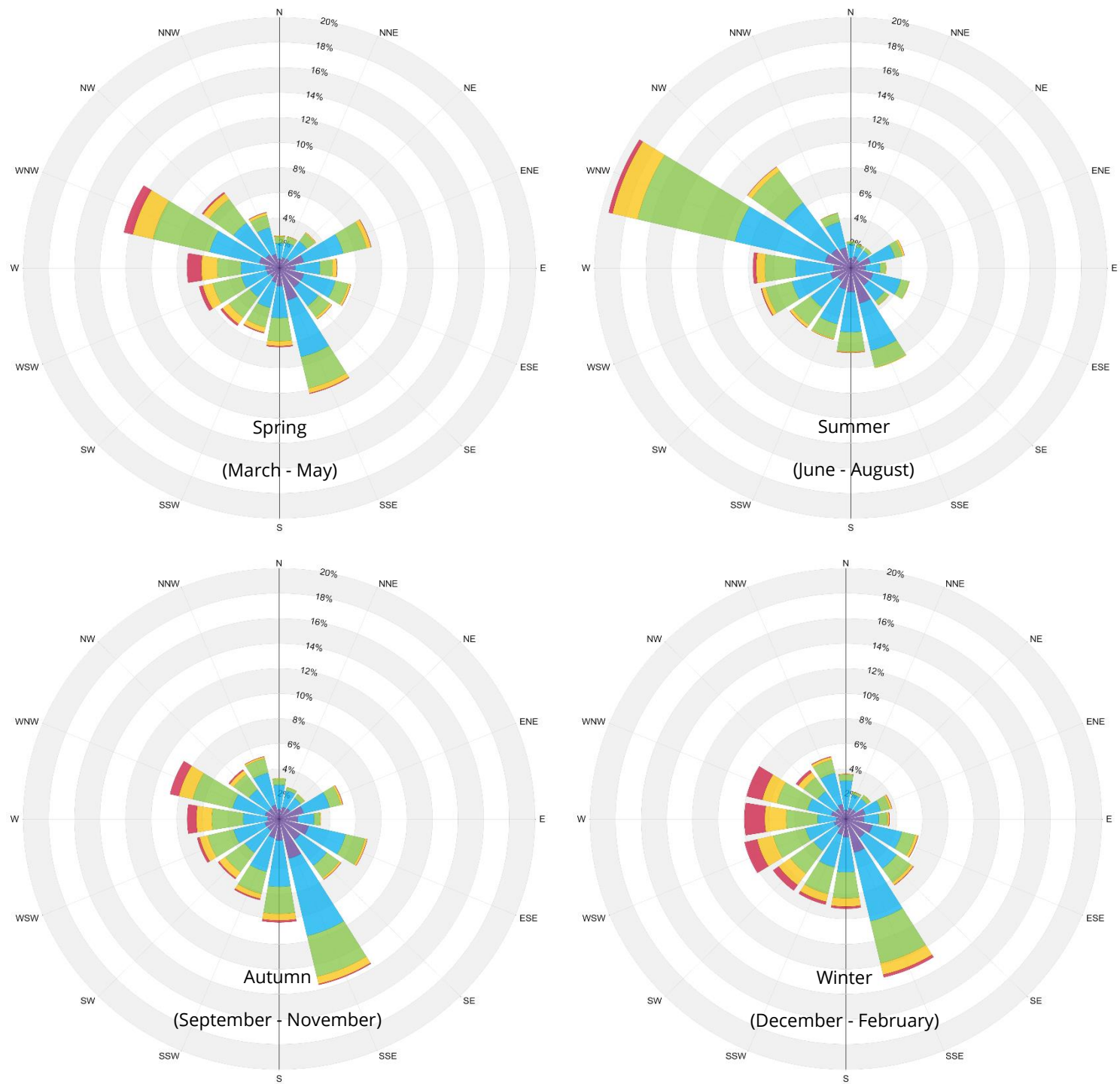
Figure 12.1 Directional Distribution (%) of Winds for Liverpool John Lennon Airport (1991-2011)
