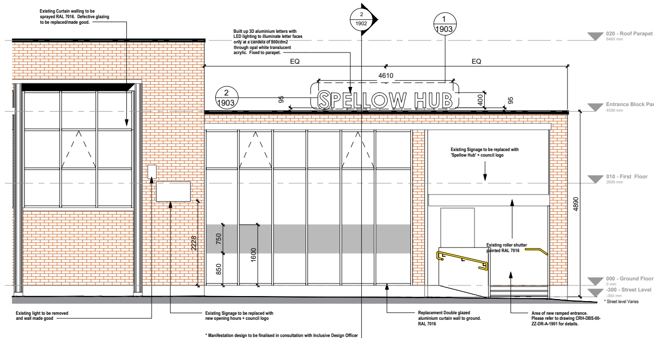
1 Proposed Elevation County Road - Signage 1 : 50
