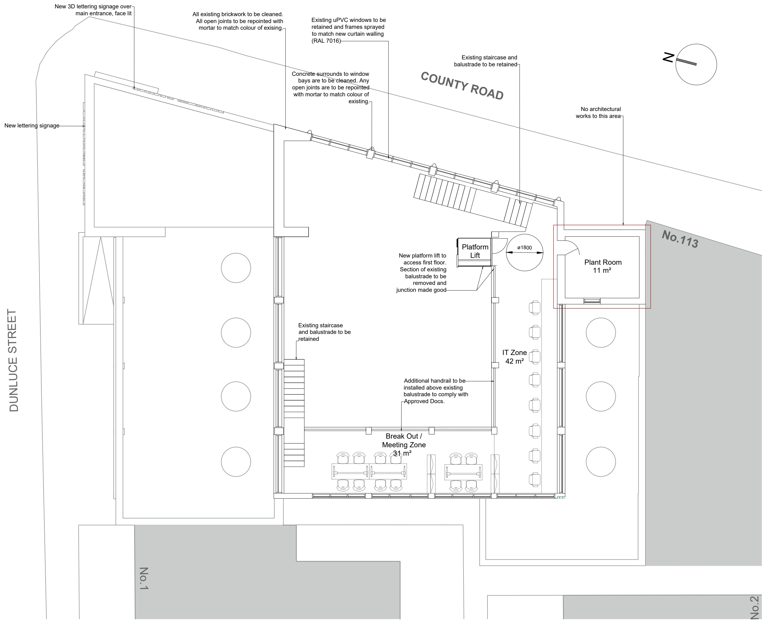
PROPOSED BALCONY / FIRST FLOOR Scale 1:100 G.I.A. : 89 sq.m.
