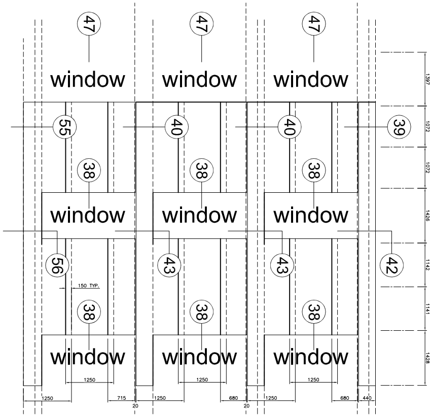
BUILT-UP ELEVATION CURVED CORNER AT GRIDS A & 9
