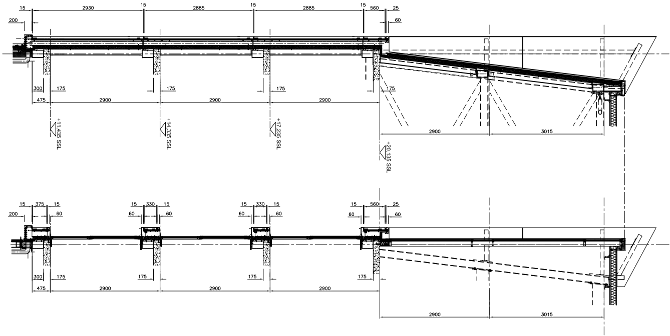
GENERAL SECTIONS
