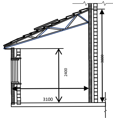
Section ZZ
