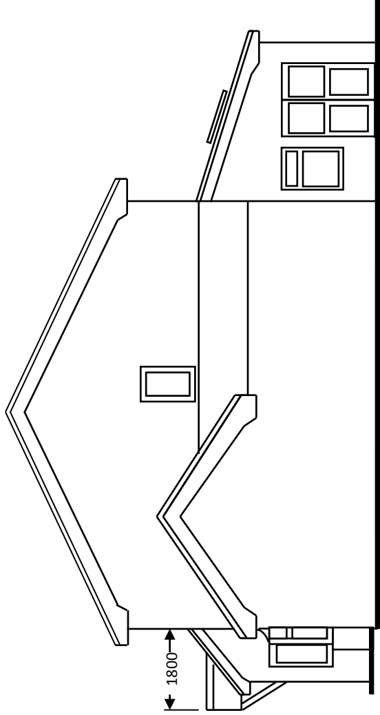
PROPOSED LEFT SIDE ELEVATION
