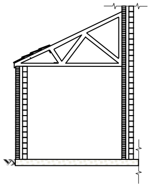
Section YY
