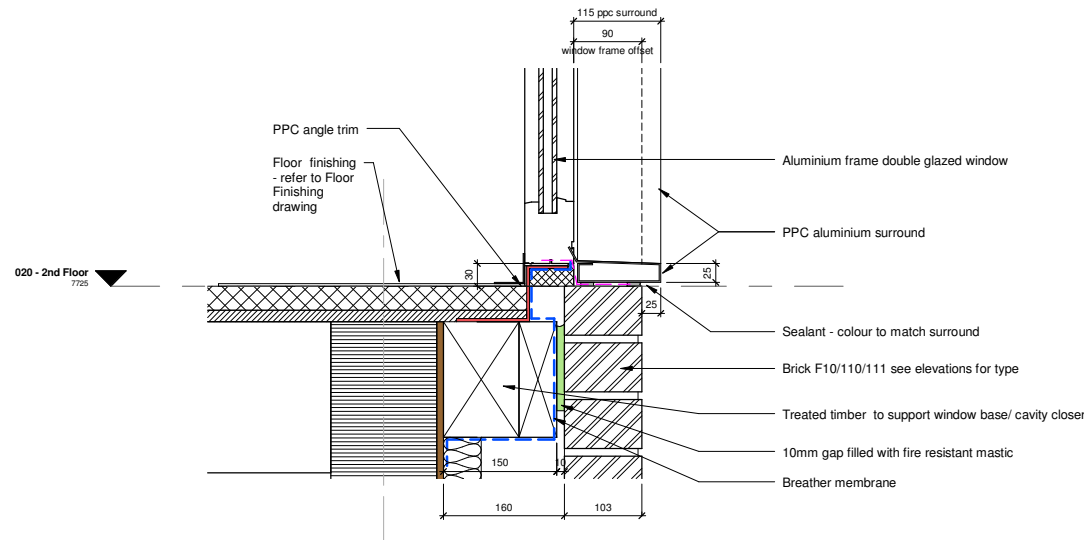
04 - Typical Detail to Front Standard Window Base (with PPC Surround) 1 : 5
