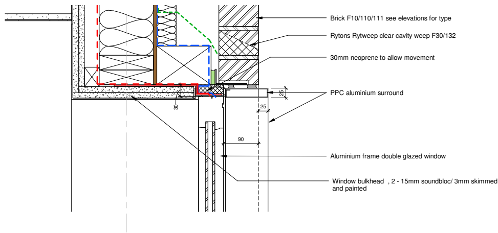
03 - Typical Detail to Front Standard Window Head (with PPC Surround) 1 : 5
