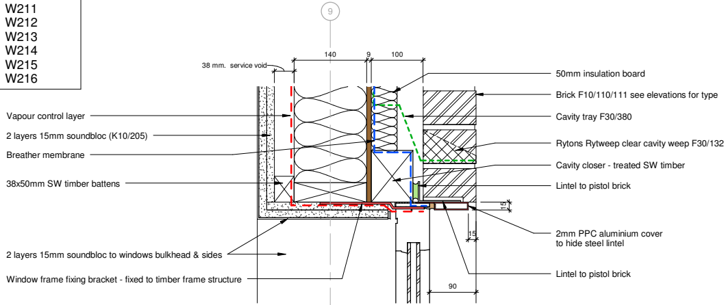
01 - Typical Detail to Standard Windows Head 1 : 5
