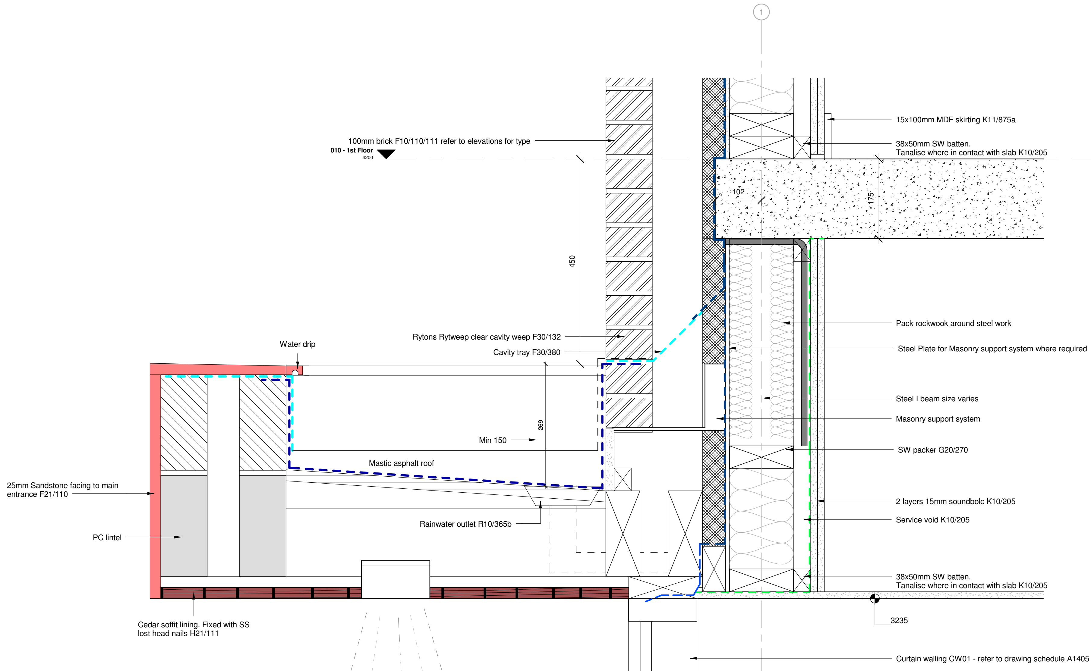
Main Entrance Canopy WIP 1 : 5
