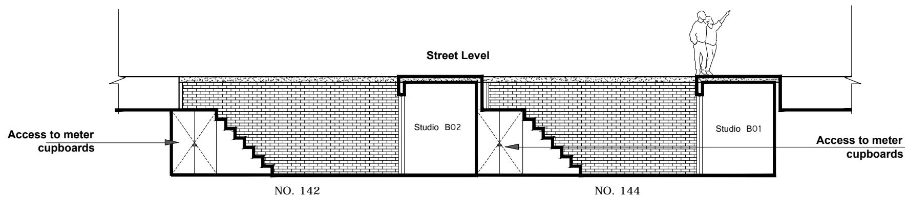
schematic section R-R showing meter cupboards
