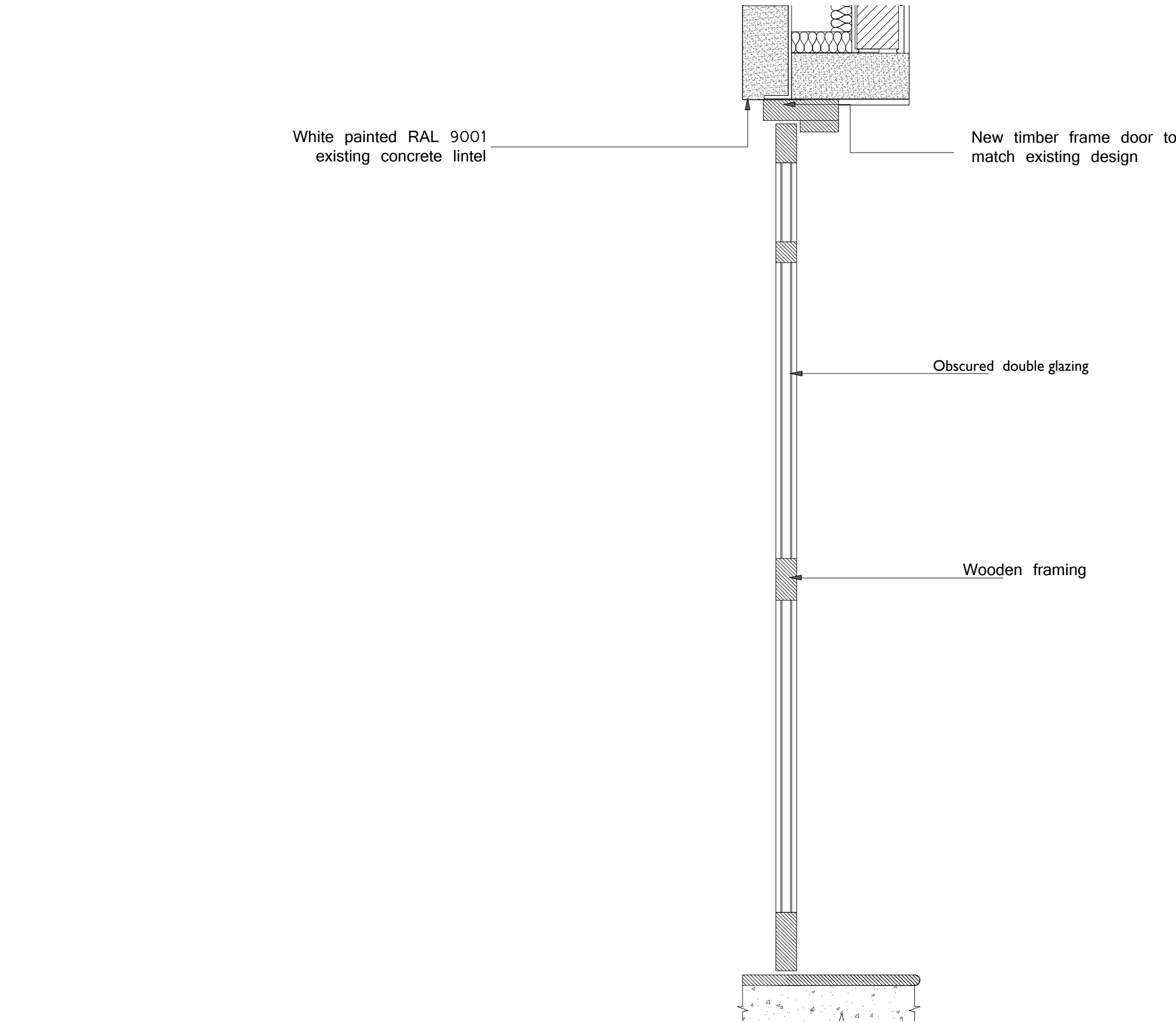
Type 3 Door detail section scale 1.10
