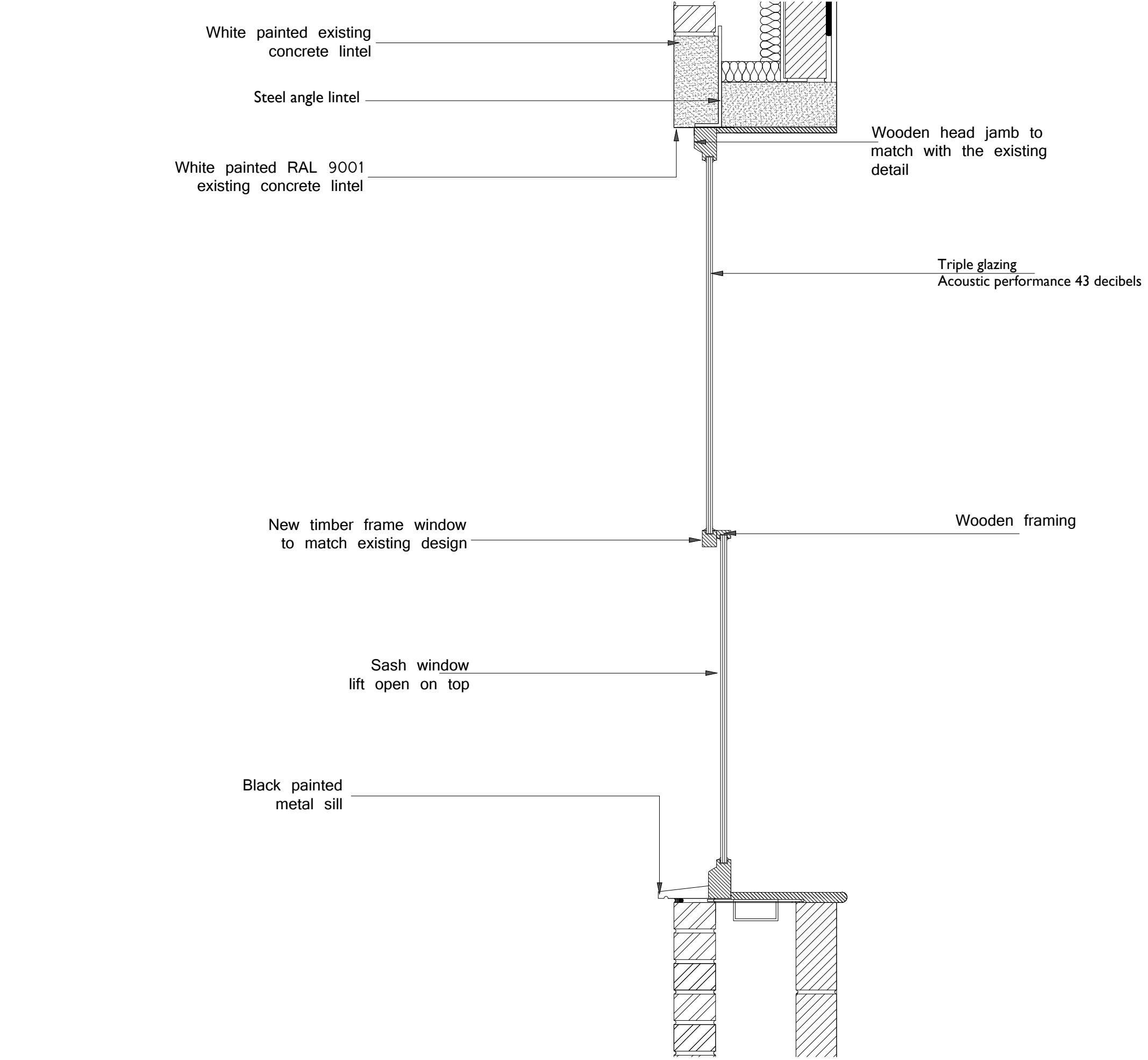
Type 5 window detail section scale 1.10
