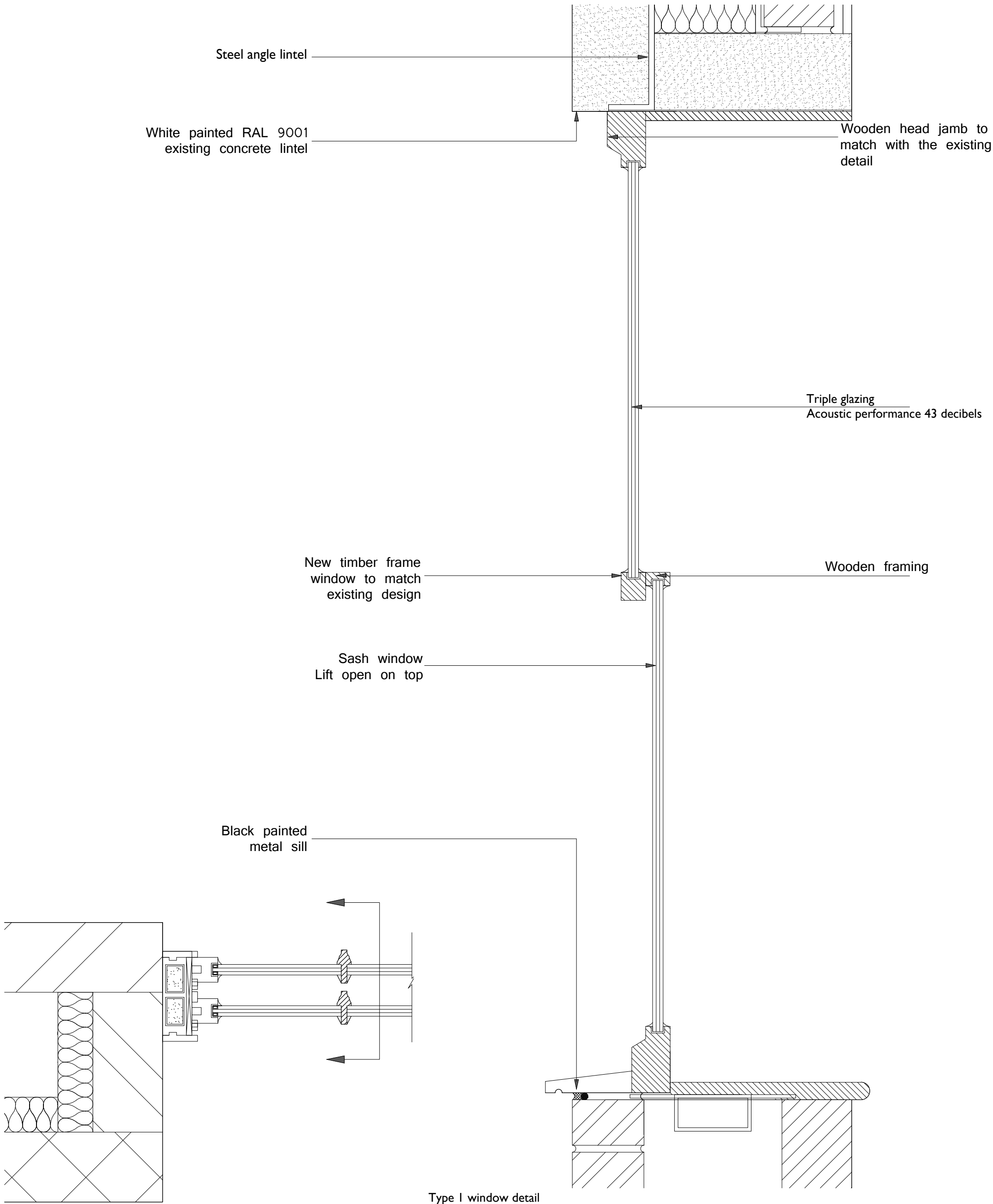
window detail plan scale 1.5 Type I window detail section scale 1.5
