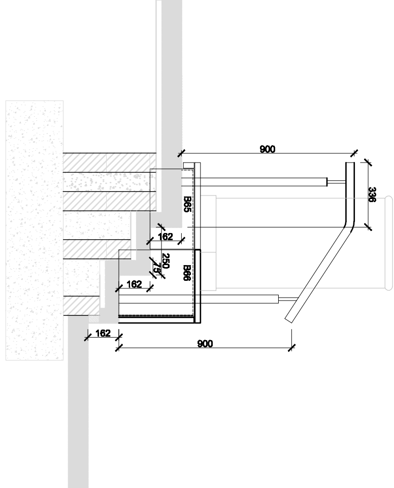
SECTION THRO STAIR
