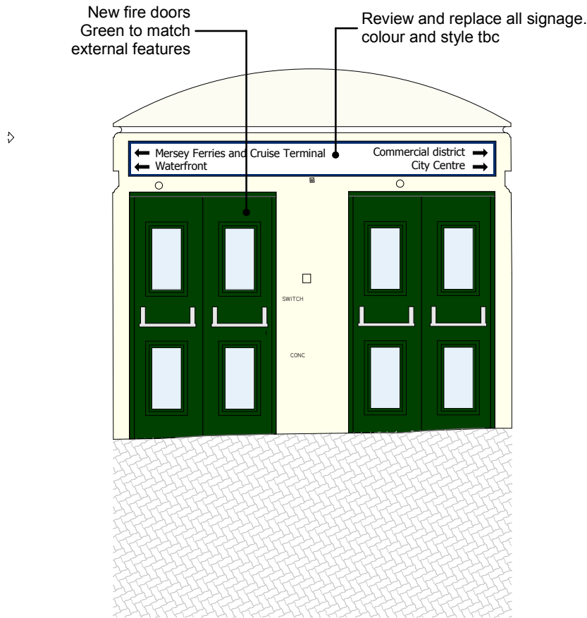
Internal Elevation
