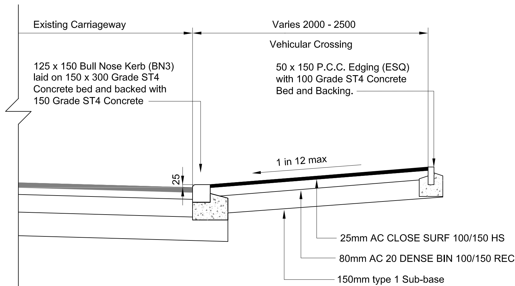
VEHICULAR CROSSING DETAIL
