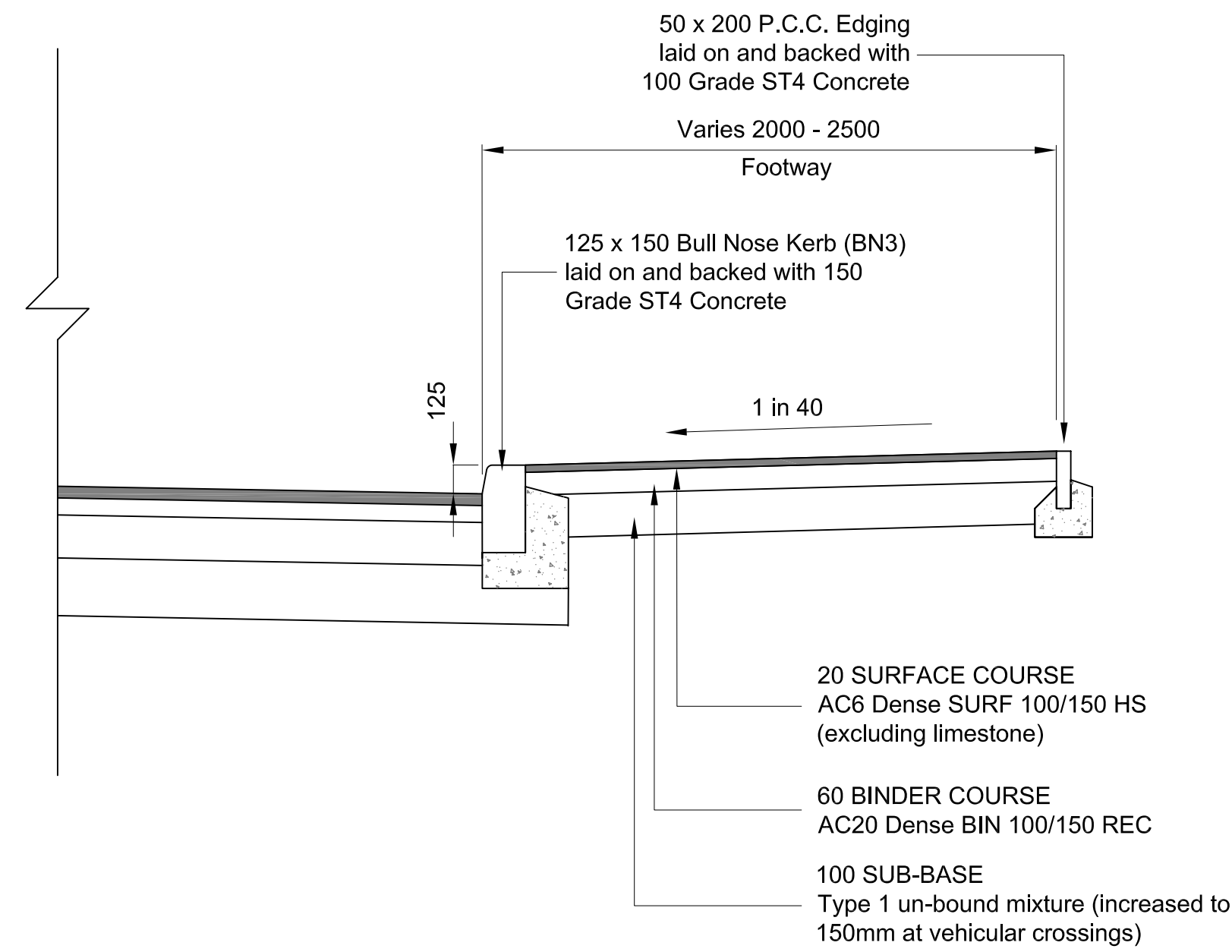
FOOTPATH DETAIL
