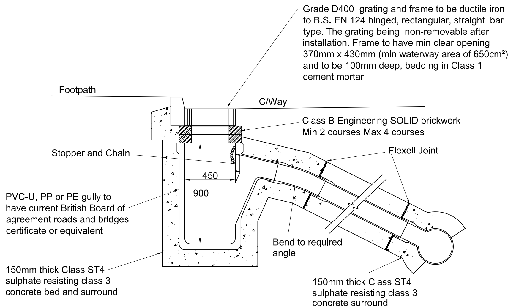
STREET GULLY TYPE 1
