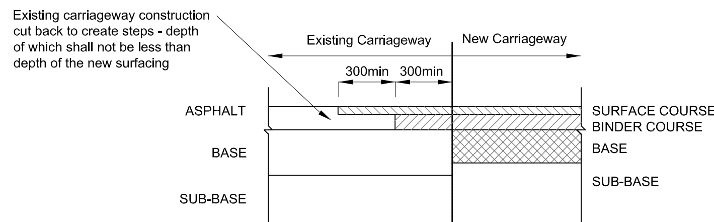
DETAIL OF TRANSVERSE JOINT BETWEEN NEW AND EXISTING CARRIAGEWAY
