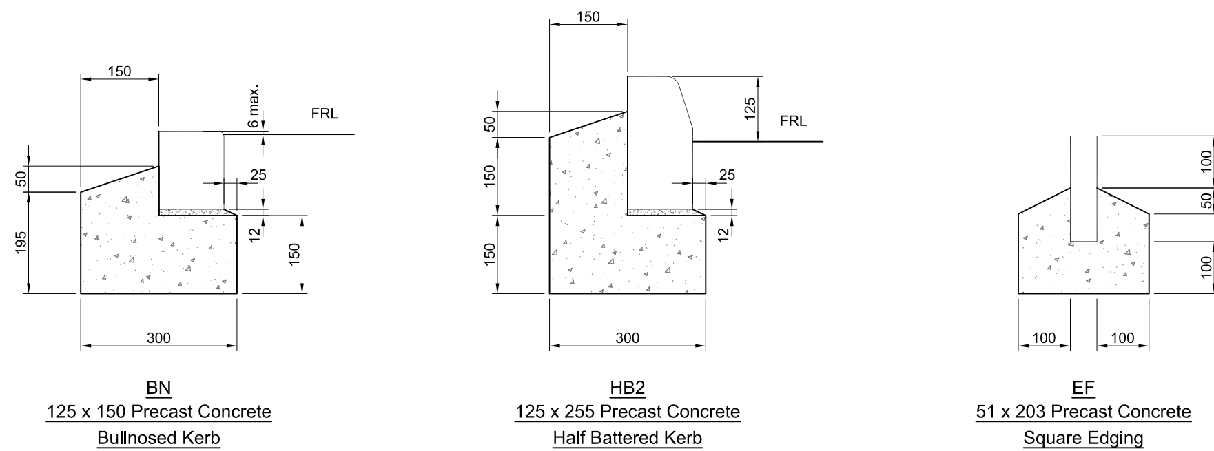
KERBING AND EDGING DETAILS
