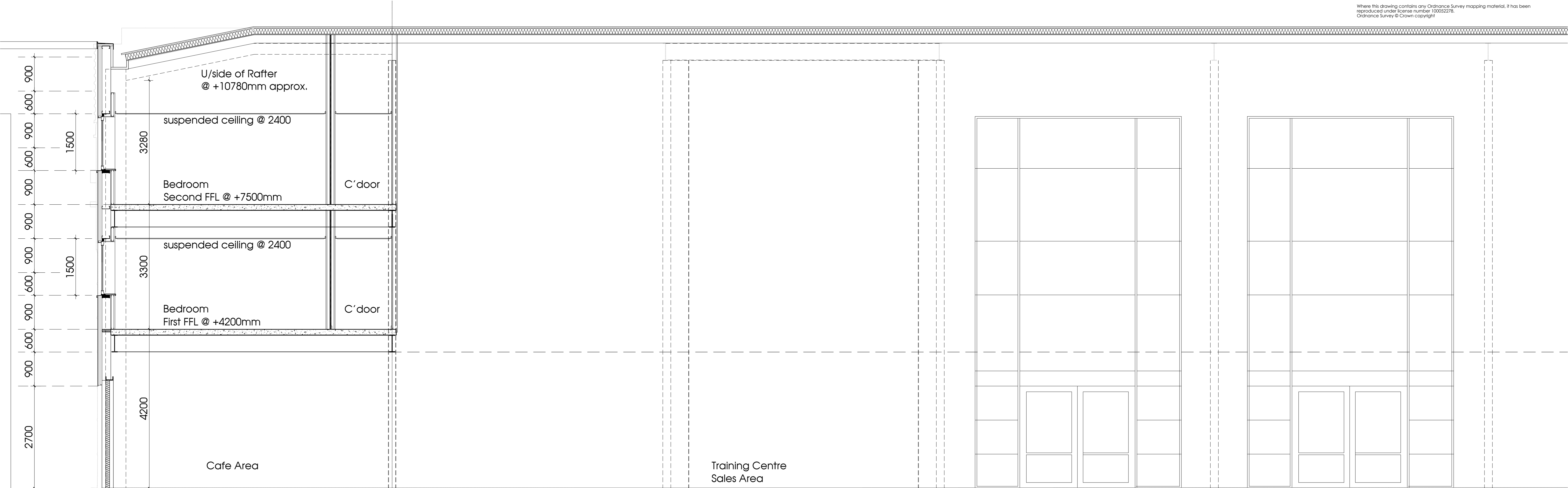
SECTION A - Indicative Section Through Accommodation/Units scale 1:50
