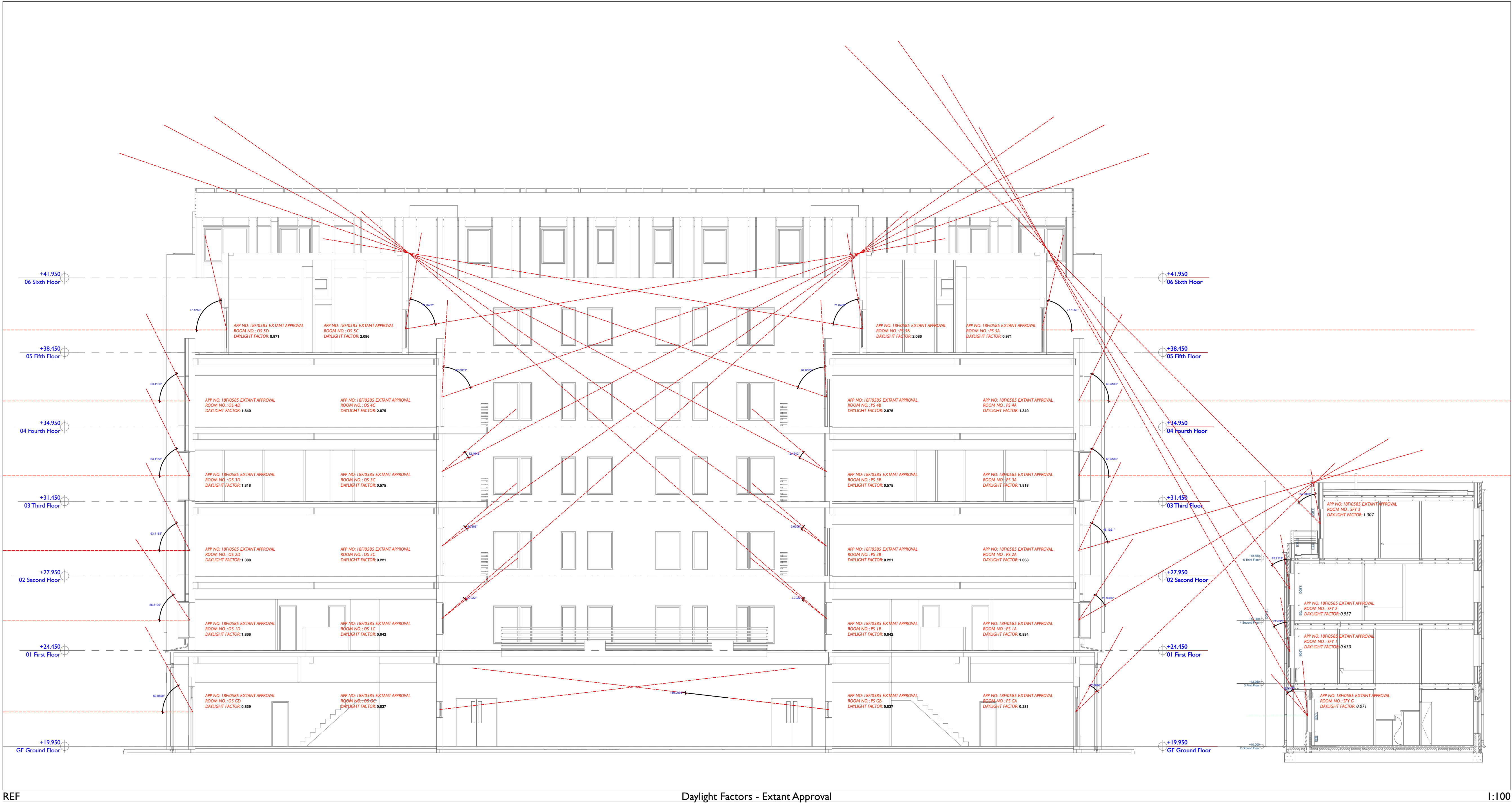
REF Daylight Factors - Extant Approval 1:100
