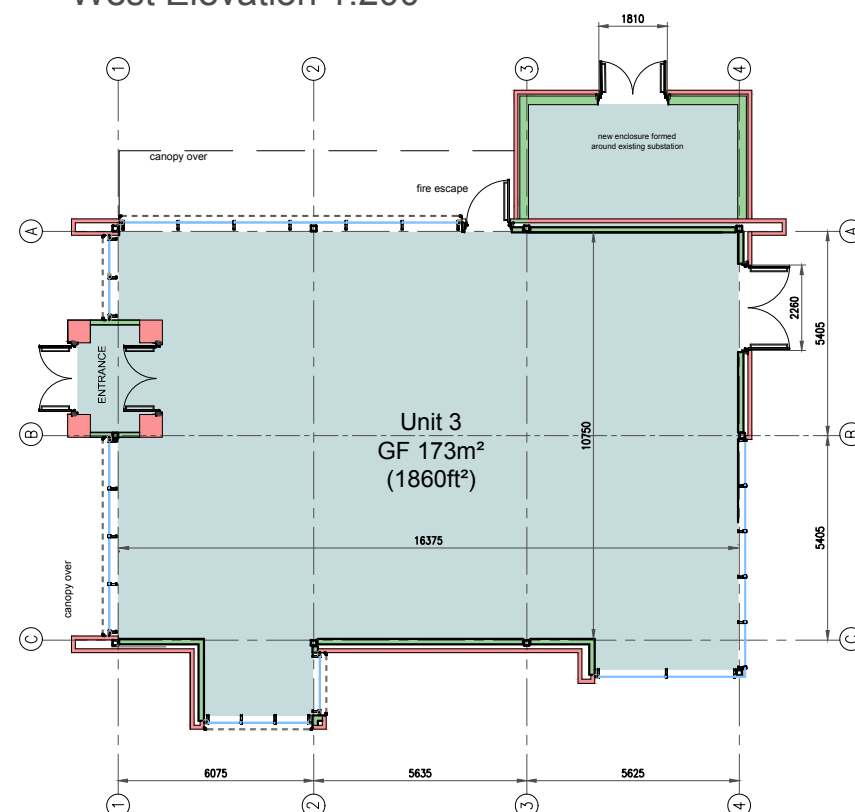
Floor Plan 1:200 @ A3
