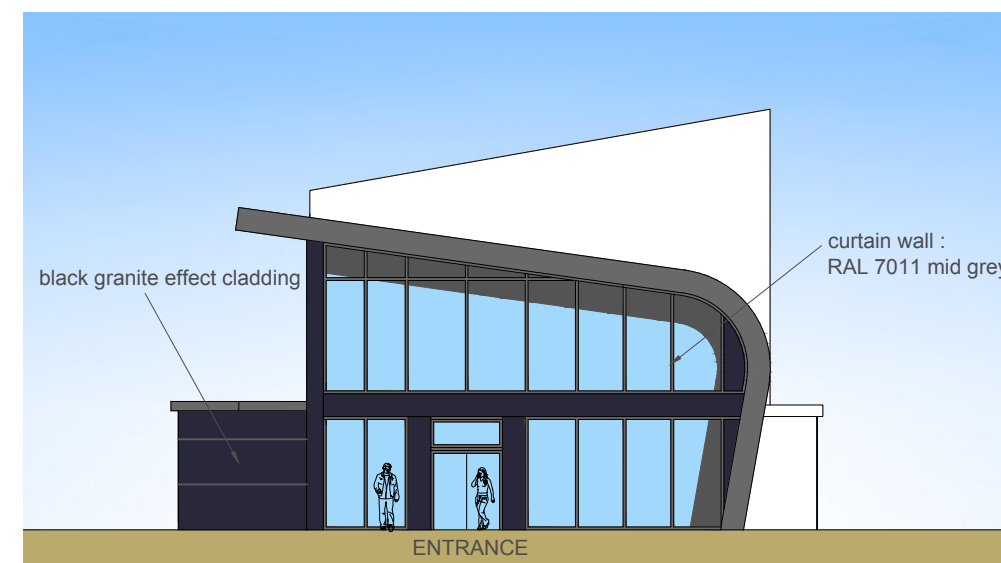
North Elevation 1:200
