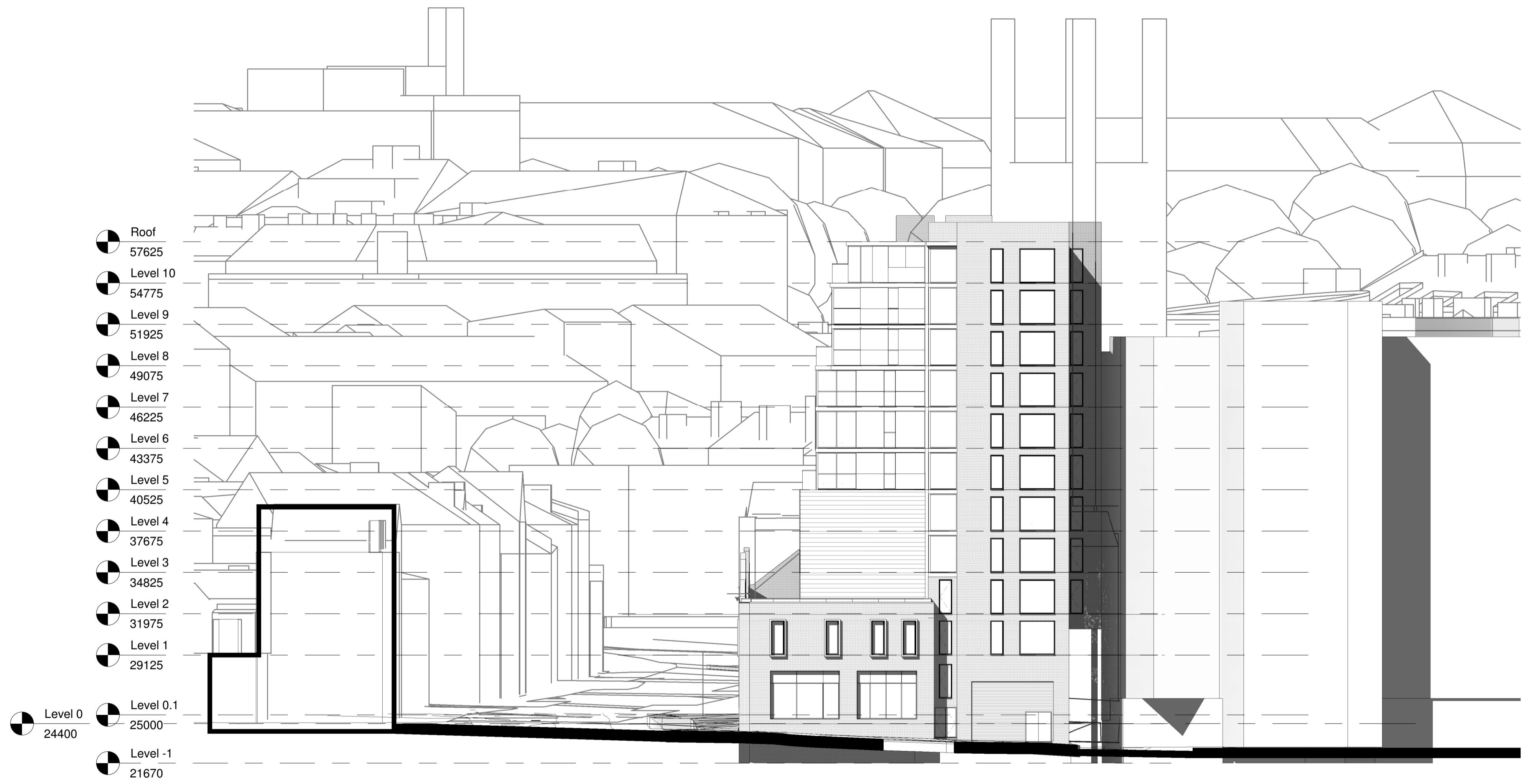
2 North Elevation-Street Scene 1 : 200
