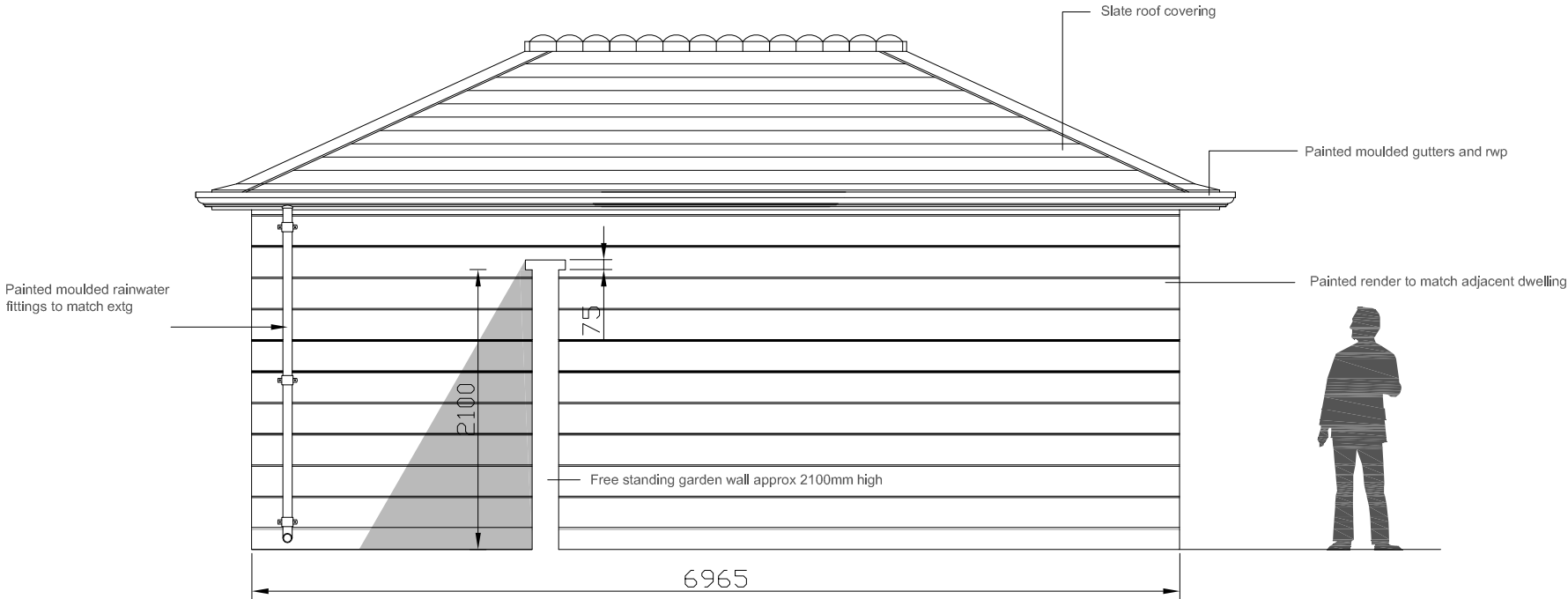
SIDE ELEVATION
