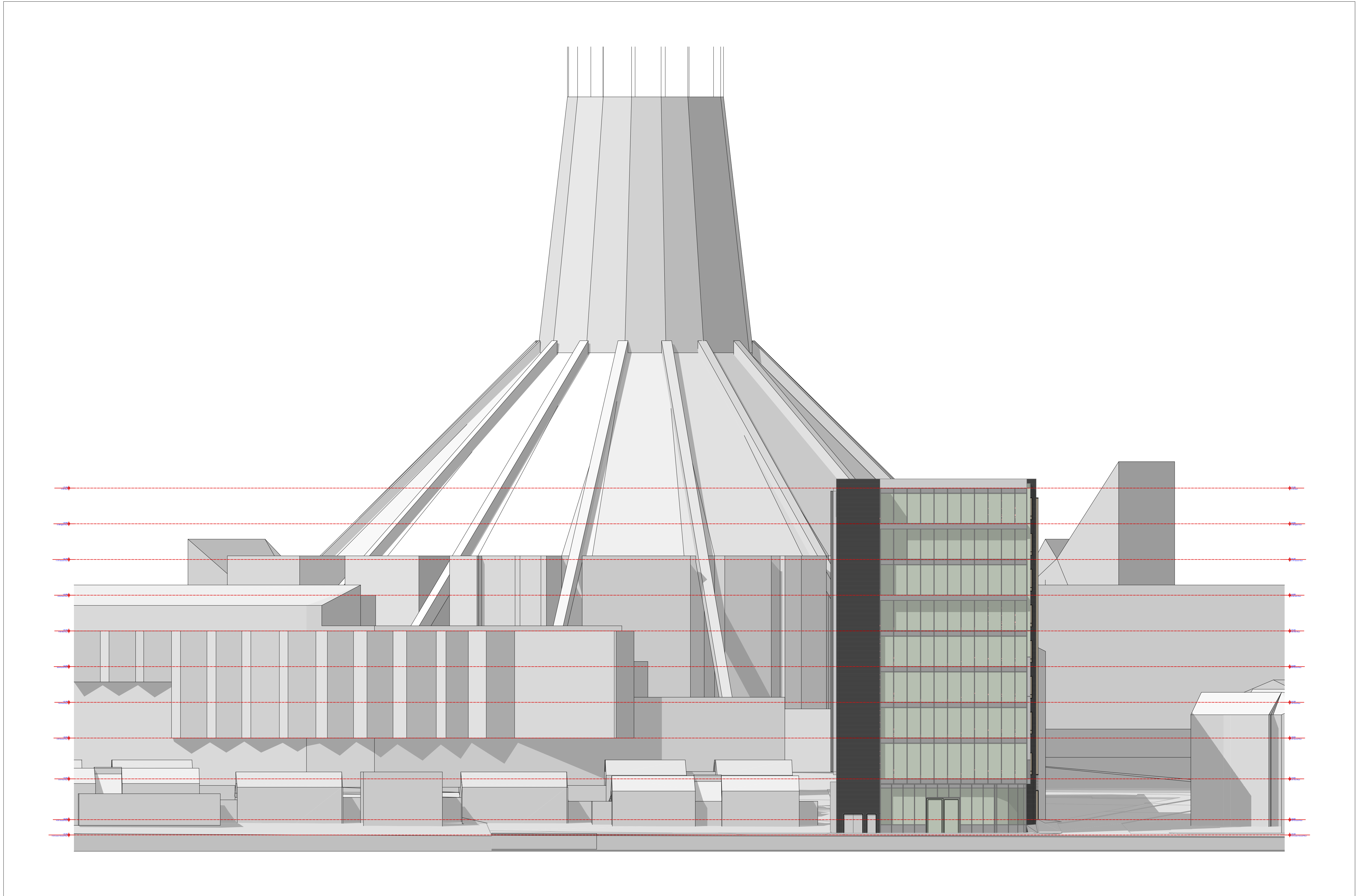
SS-02 Pomona Street Scene 1:200
