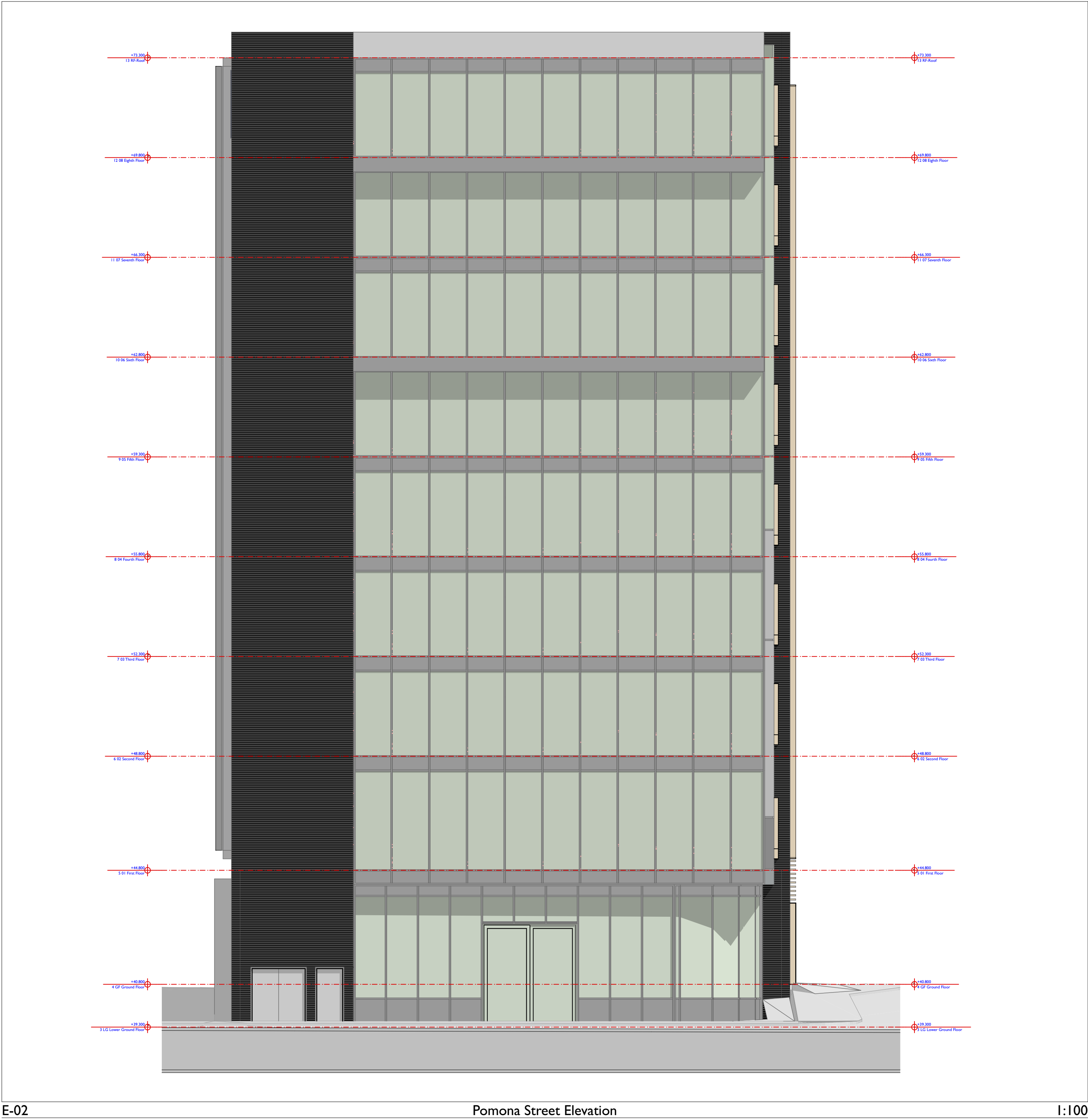
Pomona Street Elevation
