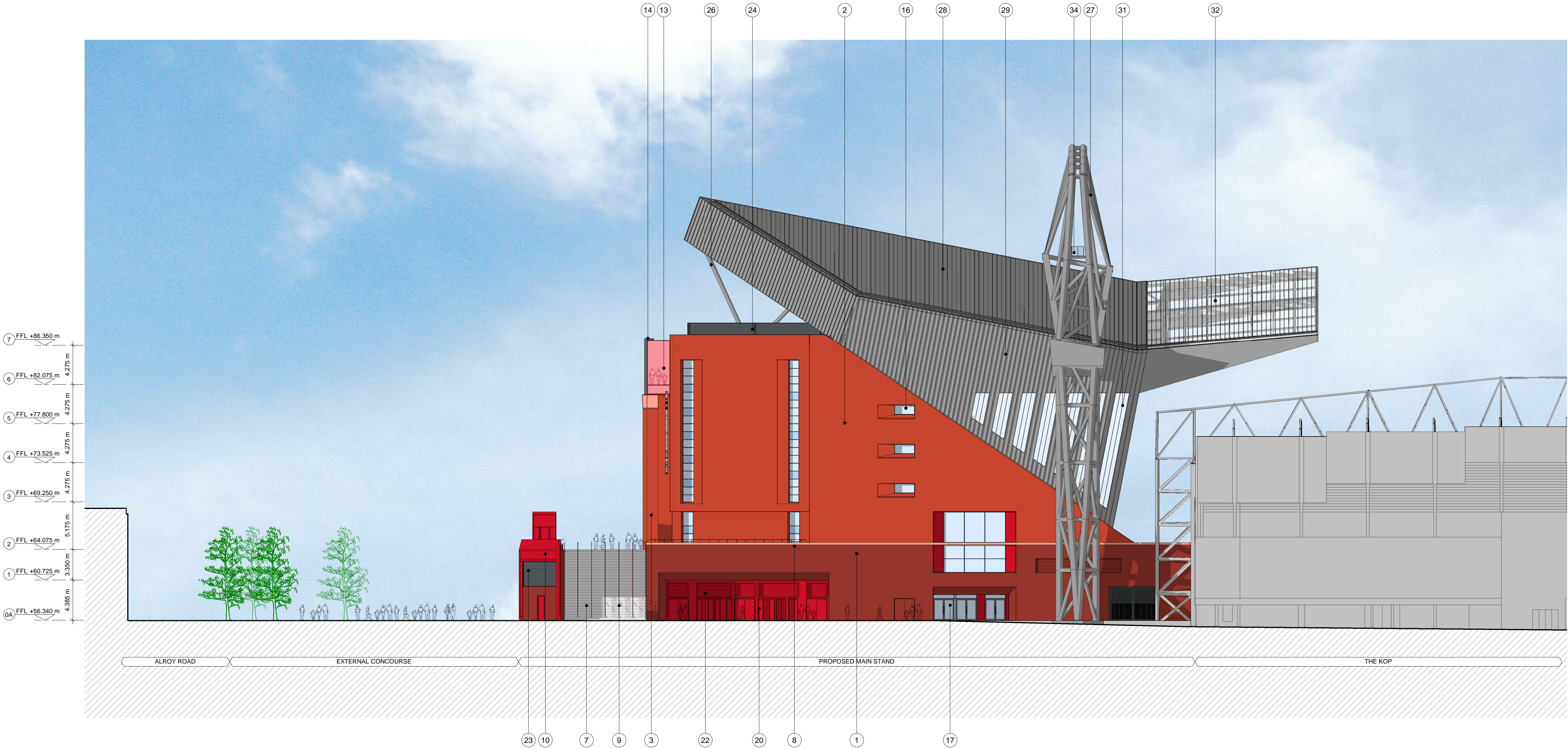
1 SOUTH WEST ELEVATION PROPOSED GENERAL ARRANGEMENT ELEVATION
