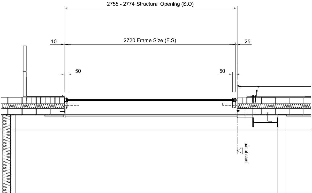
Typical Section - Street Level
